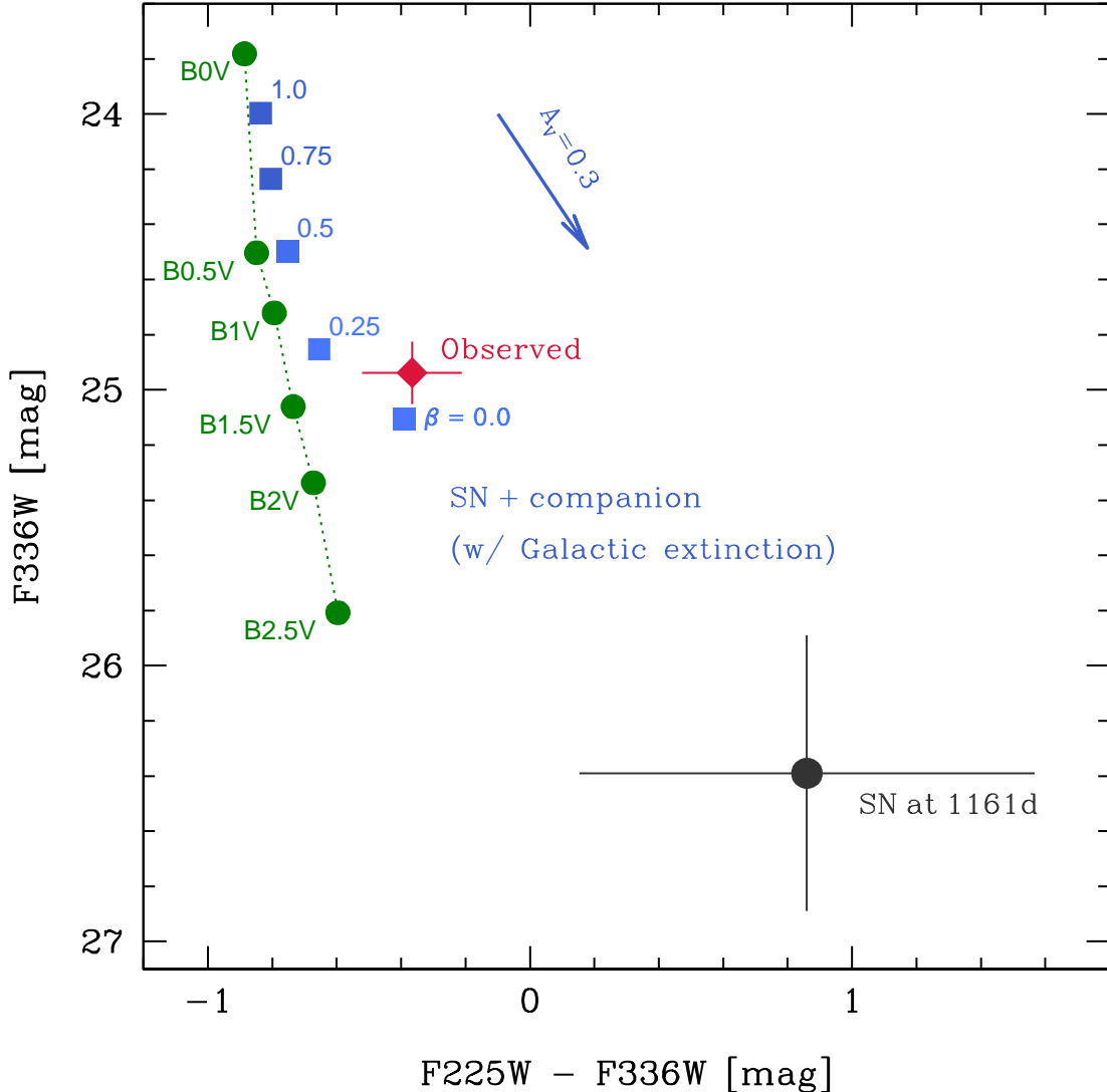
FIG. 3.— F336W versus (F225W - F336W) color-magnitude diagram. The observed object is shown with a red diamond, without correcting for extinction. The black dot shows the expected location of the SN, as estimated in Figure 2. Blue squares indicate the expected observations from the SN plus a binary companion (SN + companion) according to the models of Benvenuto et al. (2013), for varying mass-accretion efficiency ( \beta ; labeled next to each point). A distance of 7.8 Mpc was adopted, and the SN + companion model photometry was reddened by Galactic extinction of A_V = 0.10 mag to reproduce the observations. Green dots show the location of main sequence stars for the same distance and reddening. The arrow indicates the reddening vector for an additional extinction of A_V = 0.3 mag that may be produced by dust in M51 (see the text for details).
