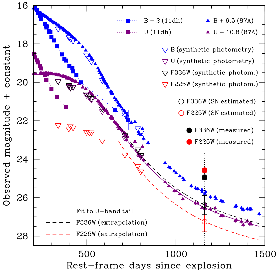
FIG. 2.— Estimated brightness of the fading SN. Squares indicate the U - and B -band light curves of SN 2011dh from Ergon et al. (2014b). Filled triangles show the light curves of SN 1987A (Hamuy & Suntzeff 1990; Walker & Suntzeff 1991) shifted to match the evolution of SN 2011dh (see text). Open triangles show the synthetic photometry in the HST bands computed from spectra of SN 1987A (Pun et al. 1995) and shifted to the scale of SN 2011dh. The solid curve is a fit to the late-time decline of the U -band light curve of SN 1987A. Dashed curves are the same fit, shifted vertically to match the synthetic light curves in F225W and F336W bands. The vertical dotted line indicates the epoch of our HST observations where the SN brightness was estimated from the shifted decline fits.
