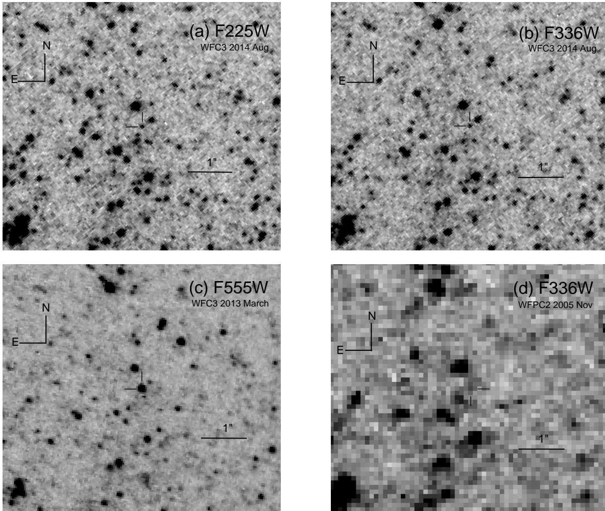
FIG. 1.— (a) and (b) Portions of the deep F225W- and F336W-band images obtained with the HST and WFC3/UVIS on 2014 August 7.2 UT. (c) 2013 March image obtained with WFC3/UVIS and filter F555W showing the fading SN ejecta (Van Dyk et al. 2013). (d) Pre-explosion image obtained with the WFPC2 on 2005 November showing the progenitor detection (Maund et al. 2011; Van Dyk et al. 2011). Images in all four panels are centered at the SN location and scale and orientation are indicated. A point source is detected in both near-UV images from 2014 August, as indicated with tick marks. The position of the source is coincident with that of the SN in the 2013 March image to a projected distance of \lesssim 0.15 pc.
