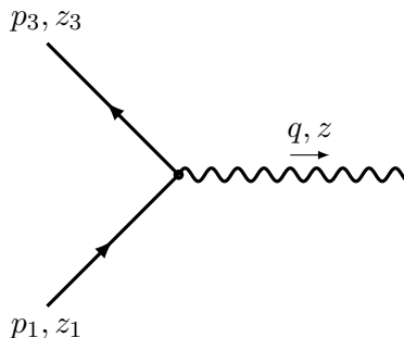
Figure 4. The three-point interaction between two elementary particles with spin J and a graviton.
