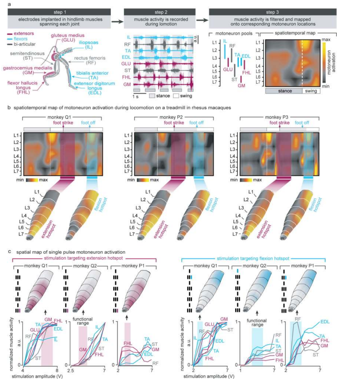
Extended Data Figure 3. Anatomical, computational, and functional experiments allowed the identification of stimulation protocols to access flexion and extension hotspots
