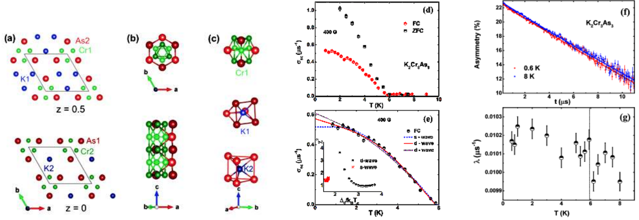
FIG. 9: (a) Illustration of the crystal structure of \text{K}_2\text{Cr}_3\text{As}_3 . (b) Crystal structure of the [(\text{Cr}_3\text{As}_3)^{2-}]_\infty tubes, which are major structural units in the \text{A}_2\text{Cr}_3\text{As}_3 materials. (c) Illustration showing the chemical bonding of Cr1 (top), K1 (middle), and K2 (bottom). (a)-(c) are reprinted from J. Bao et al. Phys. Rev. X 5 , 011013 (2015) 82 . Available under a Creative Commons Attribution 3.0 License. (d) Muon depolarization rate \sigma_{sc}(T) as function of temperature for \text{K}_2\text{Cr}_3\text{As}_3 for a field of 400 G with both zero-field and field-cooling. (e) \sigma_{sc}(T) for field-cooled measurements where the lines display fits for different gap models. The short-dashed (blue) line shows the fit using an isotropic single-gap s -wave model and the solid (red) line and dotted (purple) lines show fits to a d -wave model. The inset shows \chi^2 vs \Delta(0)/k_B T_c . (f) ZF- \mu SR asymmetry spectra for \text{K}_2\text{Cr}_3\text{As}_3 at 0.6 K (red) and 8 K (blue), where the lines show fits to the data. (g) Electronic relaxation rate as a function of temperature, where T_c = 5.8 K is shown by the dotted vertical line. (d)-(g) are reprinted with permission from Adroja et al. Phys. Rev. B 92 , 134505 (2015) 96 . Copyright 2015 by the American Physical Society.
