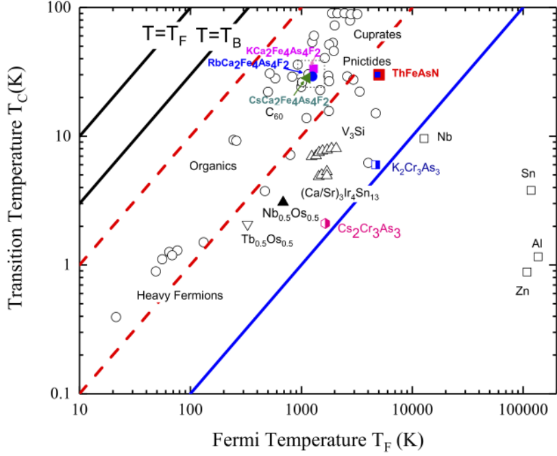
FIG. 11: Uemura plot of T_c vs. effective Fermi temperature T_F . The “exotic” superconductors lie within a region bounded by 1/100 \leq T_c/T_F \leq 1/10 , as indicated by the red dashed lines from Adroja et al. Phys. Rev. B 96 , 144502 (2017) 146 . The solid black line corresponds to the Bose-Einstein condensation temperature ( T_B ). The positions of ACa_2Fe_4As_4F_2 ( A = K, Rb and Cs ) and ThFeAsN on the plot place these materials as being exotic superconductors 146 .
