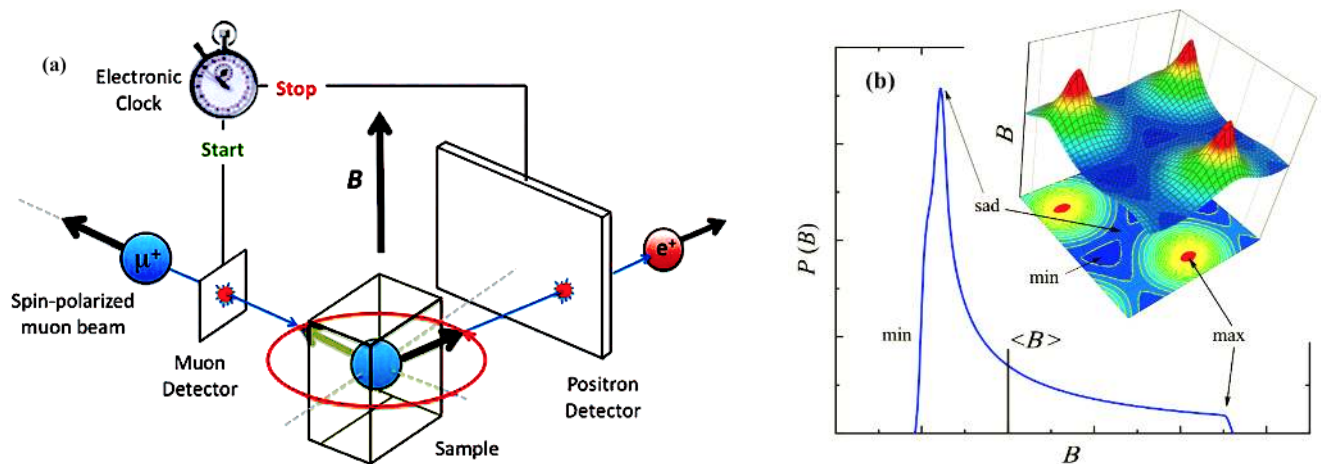
FIG. 4: Schematic representation of a \mu SR experiment. (a) Illustration of the transverse field \mu SR experimental setup. After the spin-polarized muons are implanted in the sample, the number of decay positrons detected in the forward and backward detectors is counted as a function of time from Iain McKenzie, Annu. Rep. Prog. Chem., Sect. C: Phys. Chem. 109 , 65–112 (2013) 107 . (b) Field distribution of a regular triangular flux-line lattice, with the minimum ( B_{min} ), maximum ( B_{max} ), and saddle point ( B_{sad} ) fields indicated by the arrows. Both panels are reprinted with permission from Khasanov et al. Supercond. Sci. Technol. 28 034003 (2015) 108 . Copyright 2015, the Institute of Physics.
