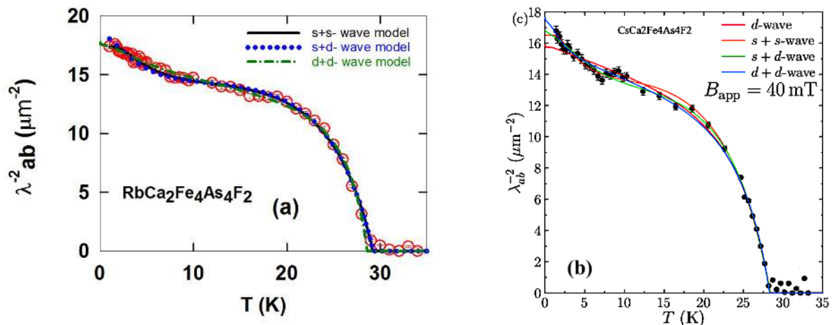
FIG. 6: (a) Variation of the square of the inverse in-plane penetration depth \lambda_{ab}^{-2}(T) with temperature for \text{RbCa}_2\text{Fe}_4\text{As}_4\text{F}_2 from Adroja et al. arXiv:1802.07334 109 . The solid and dotted lines represent the fits using different models of the superconducting gap. (b) \lambda_{ab}^{-2}(T) of \text{CsCa}_2\text{Fe}_4\text{As}_4\text{F}_2 reprinted with permission from Kirschner et al. Phys. Rev. B 97 , 060506(R) (2018) 133 . Copyright 2018 by the American Physical Society. Fits using different models with d -, (s + s) -, (s + d) -, and (d + d) -wave superconducting gap structures are also shown.
