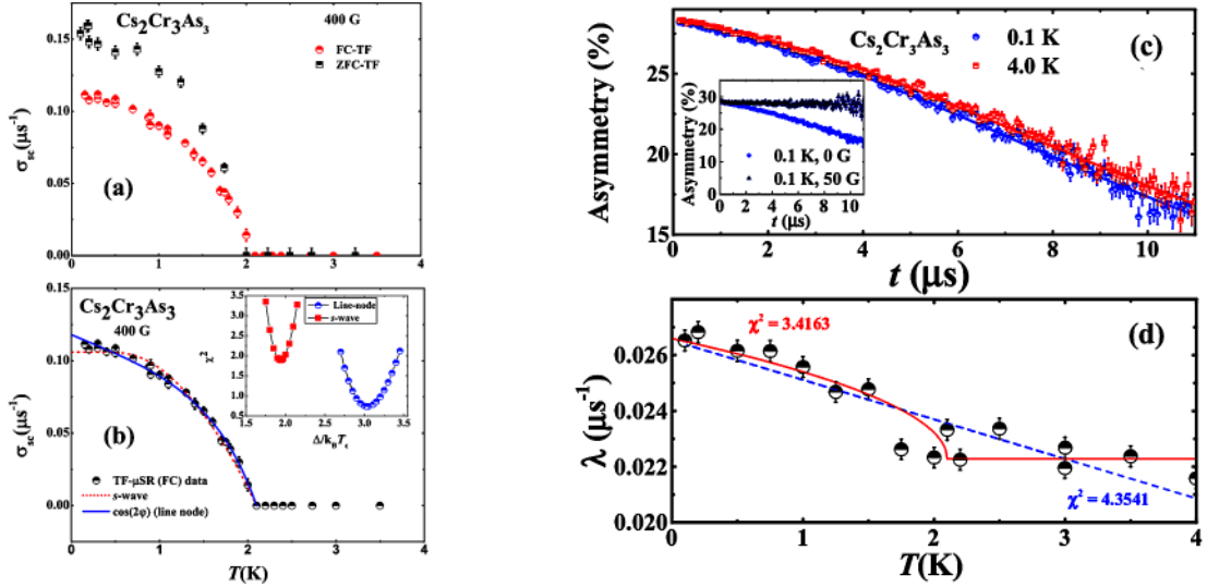
FIG. 10: (a) Temperature dependence of the superconducting component of the Gaussian relaxation rate from TF- \mu SR measurements of \text{Cs}_2\text{Cr}_3\text{As}_3 in 400 G, for both zero-field and field cooling. (b) shows the field-cooled data, which has been fitted with both s -wave and nodal models for the superconducting gap. (c) ZF- \mu SR asymmetry spectra collected at 0.1 K (circles) and 4.0 K (red squares) together with lines representing least squares fits to the data. The inset shows the asymmetry spectra in a 50 G longitudinal field together with ZF field results for comparison. (d) Temperature dependence of the electronic relaxation rate, where the dotted line marks T_c = 2.1 K. The blue dotted line shows a linear fit and the solid red line shows a BCS-type function with T_c = 2.1 K fixed from the \chi(T) data. All panels reprinted from Adroja et al. J. Phys. Soc. Jpn. 86 , 044710 (2017) 100 . Copyright 2017 by the Physical Society of Japan.
