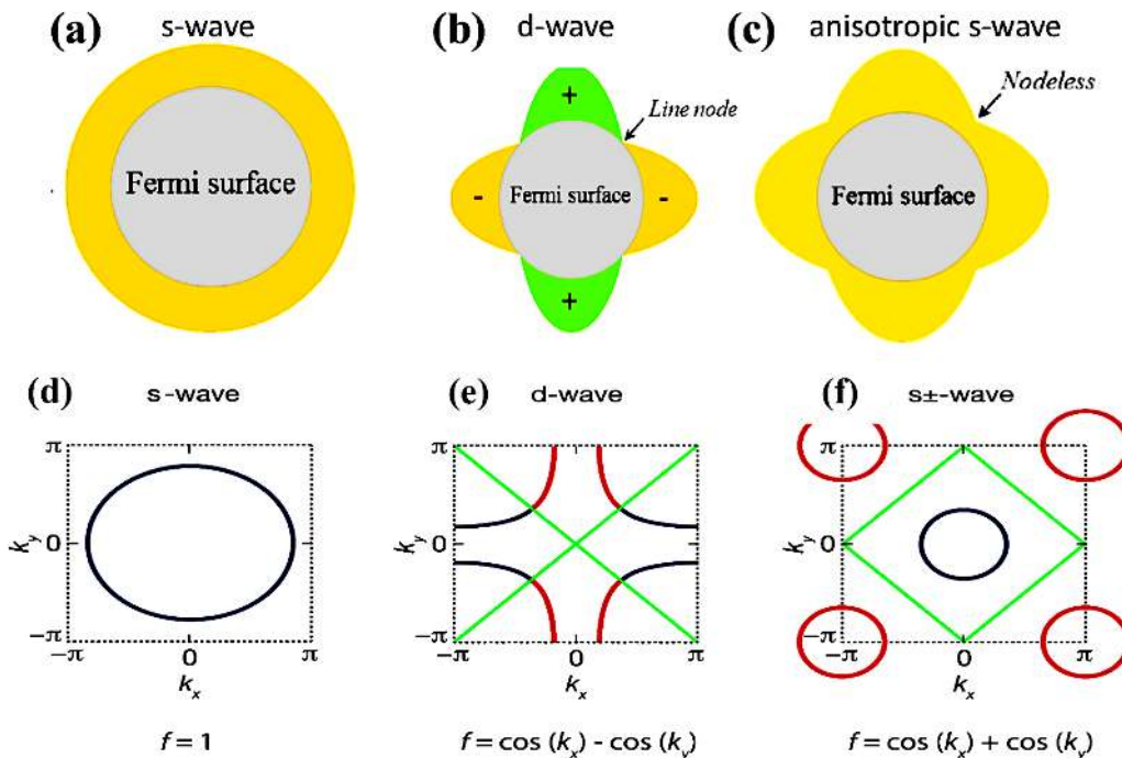
FIG. 3: (a-c) Illustrations of the superconducting gap structures corresponding to various gap symmetries, from P. K. Biswas (unpublished). (d-f) Schematic drawings of two dimensional Fermi surfaces and the Brillouin zones from Tegel 110 , where the green lines indicate the nodes in the superconducting order parameter and the blue/red circles highlight the different signs of the superconducting order parameter.
