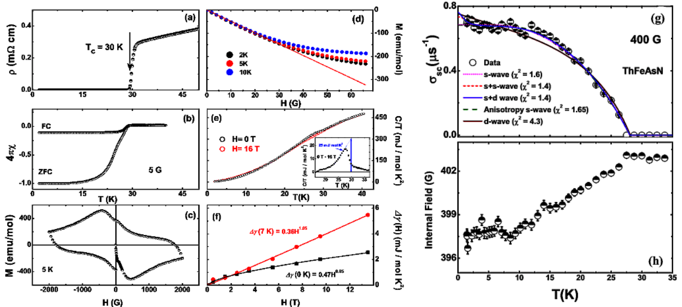
FIG. 7: (a) Resistivity of ThFeAsN as a function of temperature. (b) \chi(T) vs. T in zero-field cooled (ZFC) and field cooled (FC) modes with an external applied field of 5 G. (c) Isothermal field dependence of the magnetization at 5 K performed upon sweeping the field to positive and negative fields. (d) Isothermal M(H) at 2, 5 and 10 K. (e) Temperature dependence of the heat capacity in zero-field and 16 T. The inset of (e) shows the difference of the heat capacity data between the two datasets plotted as C/T vs T . The blue vertical arrow shows the heat capacity jump. (f) Variation of the electronic specific heat coefficient \Delta\gamma ( =\gamma(H)-\gamma(0) ) with field extrapolated to T\sim 0 K and 7 K. The solid red line shows a power law fit, \gamma(H)\sim H^n . (g) Muon depolarization rate \sigma_{sc}(T) as function of temperature for ThFeAsN cooled in a field of 400 G, after subtracting the nuclear contribution. The lines correspond to fits of the data using various models of the superconducting gap. The dotted magenta line shows the fit using an isotropic single-gap s -wave model, the dashed red line and blue solid line show the fits to the two-gap models s+s wave and s+d wave, respectively. The green long-dashed line represents the fit using an anisotropic s -wave model, and the solid purple line shows the fit using the d -wave model. (h) Temperature dependence of the internal field of ThFeAsN from TF- \mu SR. All panels reprinted with permission from Adroja et al. Phys. Rev. B 96 , 144502 (2017) 146 . Copyright 2017 by the American Physical Society.
