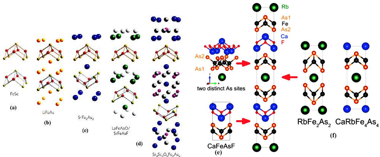
FIG. 1: Illustration of the different crystal structures of the parent compounds of various FeSCs, (a) 11-type, (b) 111-type, (c) 122-type and (d) 1111-type and 32522-type materials. Reprinted with permission from Paglione et al. Nature Physics 6, 645 (2010) 19 . Copyright 2010 by Springer Nature. (e) and (f) represent the tetragonal crystal structure of newly discovered ACa_2Fe_4As_4F_2 ( A = K, Rb and Cs ) compounds along with those for (f) RbFe_2As_2 , CaRbFe_4As_4 and (e) CaFeAsF from Adroja et al. arXiv:1802.07334 109 .
