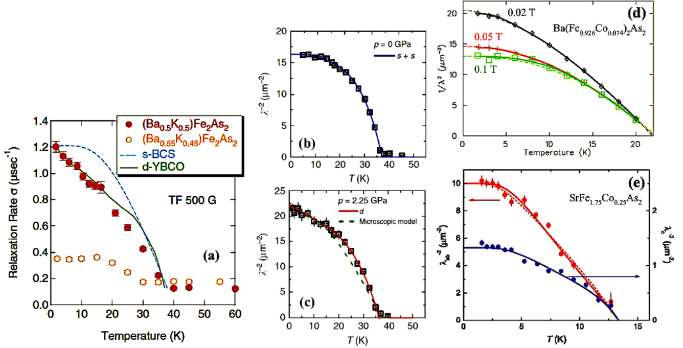
FIG. 8: (a) Temperature dependence of the muon spin relaxation rate \sigma for \text{Ba}_{0.5}\text{K}_{0.5}\text{Fe}_2\text{As}_2 and \text{Ba}_{0.55}\text{K}_{0.45}\text{Fe}_2\text{As}_2 . The dashed curve represents the isotropic gap s -wave pairing BCS superconductivity and the solid curve represents the scaled results for YBCO. Reprinted with permission from Goko et al. Phys. Rev. B 80 , 024508 (2009) 162 . Copyright 2009 by the American Physical Society. (b,c) Penetration depth \lambda (plotted as 1/\lambda^2 vs. T ) obtained from the transverse field muon spin relaxation measurements on \text{Ba}_{0.65}\text{Rb}_{0.35}\text{Fe}_2\text{As}_2 at (b) ambient pressure and (c) 2.25 GPa. The solid curve in (b) represents the fit with two-gap s -wave model and in (c) the fit according to a multiband d -wave model. The dashed line in (c) represents the fit by a microscopic model. Both (b) and (c) are reprinted from Guguchia et al. Nat. Commun. 6 , 8863 (2015) 183 . Available under a Creative Commons Attribution 4.0 International License. (d) 1/\lambda^2 vs. T obtained from the transverse field muon spin relaxation measurements on \text{Ba}(\text{Fe}_{0.926}\text{Co}_{0.074})_2\text{As}_2 . The solid curve represents the fit with two gaps ( s -wave) and the dashed line to the fit by a power-law. Reprinted with permission from Williams et al. Phys. Rev. B 80 , 094501 (2009) 168 . Copyright 2009 by the American Physical Society. (e) 1/\lambda^2 vs. T obtained from the transverse field muon spin relaxation measurements on \text{SrFe}_{1.75}\text{Co}_{0.25}\text{As}_2 . The solid curve represents the fit with two gaps ( s -wave) in the clean-limit and the dashed shows the fit in the dirty-limit. Reprinted with permission from Khasanov et al. Phys. Rev. Lett. 103 , 067010 (2009) 192 . Copyright 2009 by the American Physical Society.
