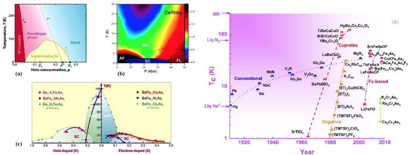
FIG. 2: Prototypical examples of the phase diagrams of three major classes of unconventional superconductors, following Bang et al. J. Phys.: Condens. Matter 29 , 123003 (2017) 114 . (a) Cuprate superconductor (YBCO) reprinted with permission from Leyraud et al. Nature 447 , 565-568 (2007) 10 . Copyright 2007 by Springer Nature. (b) Heavy fermion superconductor (CeRhIn 5 ) reprinted with permission from Park et al. Nature 456 , 366-368 (2008) 11 . Copyright 2008 by Springer Nature. (c) Fe-based 122 superconductors reprinted with permission from Liu et al. Physica C: Superconductivity and its Applications, 470 , S513-S515 (2010) 12 . Copyright 2010 by Elsevier. (d) A plot showing the historical progression of the T_c of superconductors.
