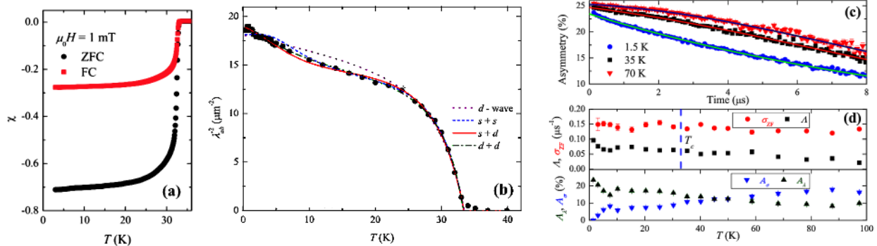
FIG. 5: (a) Magnetization as a function of temperature for \text{KCa}_2\text{Fe}_4\text{As}_4\text{F}_2 in zero-field cooled (ZFC) and field-cooled (FC) modes. (b) Variation of the square of the inverse in-plane penetration depth with temperature \lambda_{ab}^{-2}(T) for \text{KCa}_2\text{Fe}_4\text{As}_4\text{F}_2 . The lines represent fits using different models for the superconducting gap structures. The single gap d -wave and fully gapped s + s models do not fit the data well, but good fits are obtained using two-gap nodal s + d and d + d models. (c) Time dependence of zero field muon spin relaxation spectra at different temperatures for \text{KCa}_2\text{Fe}_4\text{As}_4\text{F}_2 , where the solid lines show fits consisting of sum of a Gaussian and a Lorentzian decay. (d) Variation of the Lorentzian ( \lambda ) and Gaussian ( \sigma_{ZF} ) relaxation rates with temperature, along with the corresponding amplitudes of each component. All panels are reprinted with permission from Smidman et al. Phys. Rev. B 97 , 060509(R) (2018) 130 . Copyright 2018 by the American Physical Society.
