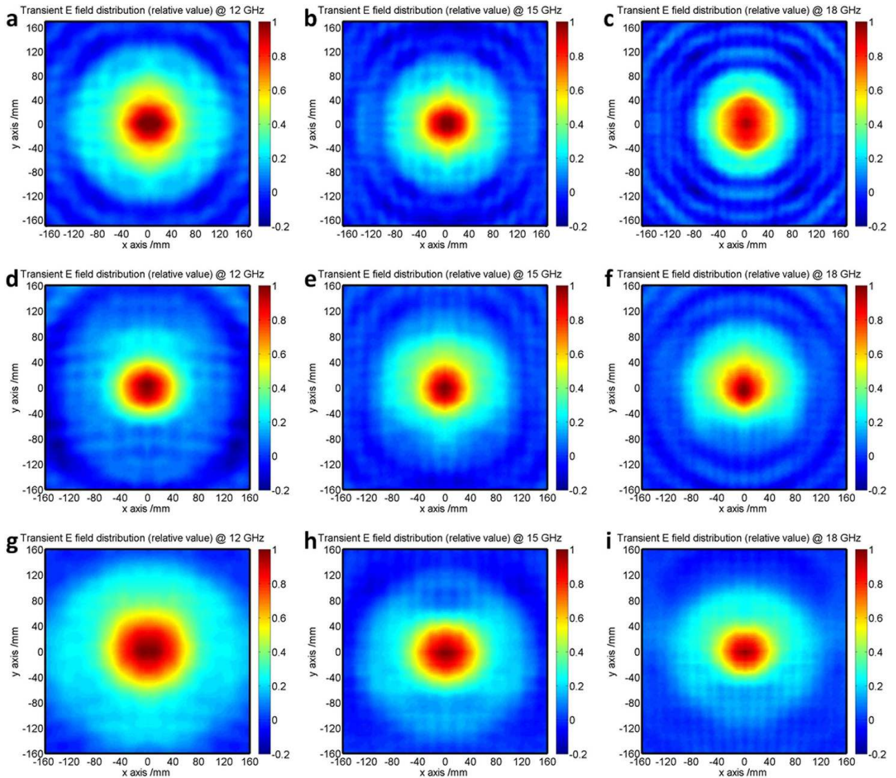
Figure 9. Experimental transversal profiles at different transverse planes at 12, 15 and 18 GHz, respectively. (a–c) z = 0.4 m. (d–f) z = 0.6 m. (g–i) z = 0.8 m.
