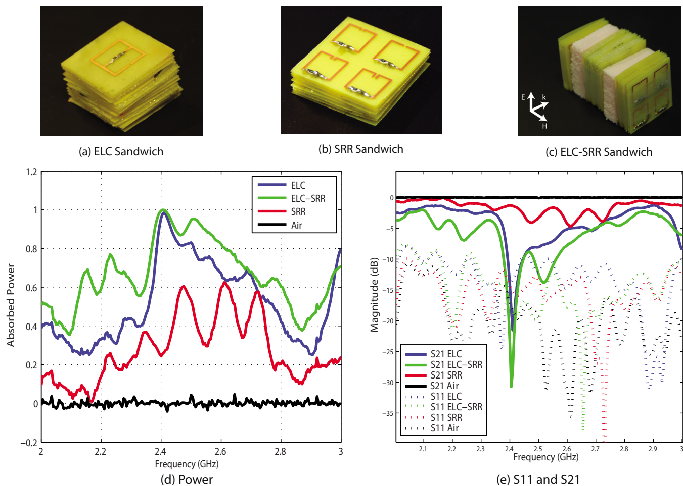
FIG. 6. (Color online) ELC-SRR sandwich experimental performance. (a) ELC sandwich. (b) SRR sandwich. (c) ELC-SRR sandwich. (d) ELC-SRR sandwich peak absorption of 99.9% at 2.4 GHz, with FWHM of 700 MHz. Distinct absorption maxima and minima are due to component particle resonances. (e) ELC-SRR sandwich absorption due to transmission (S21) decrease. S11 remains low, but varies throughout band due to imperfect matching of ELC and SRR resonances.
