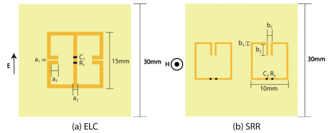
FIG. 1. (Color online) The optimum single-cell ELC-SRR absorption was achieved with (a) ELC parameters of a_1=0.35 mm, a_2=1 mm, a_3=0 mm, C_1=10 pF, and R_1=10 \Omega , and (b) SRR parameters of b_1=0.7 mm, b_2=3 mm, b_3=0.5 mm, C_2=10 pF, and R_2=5 \Omega .
