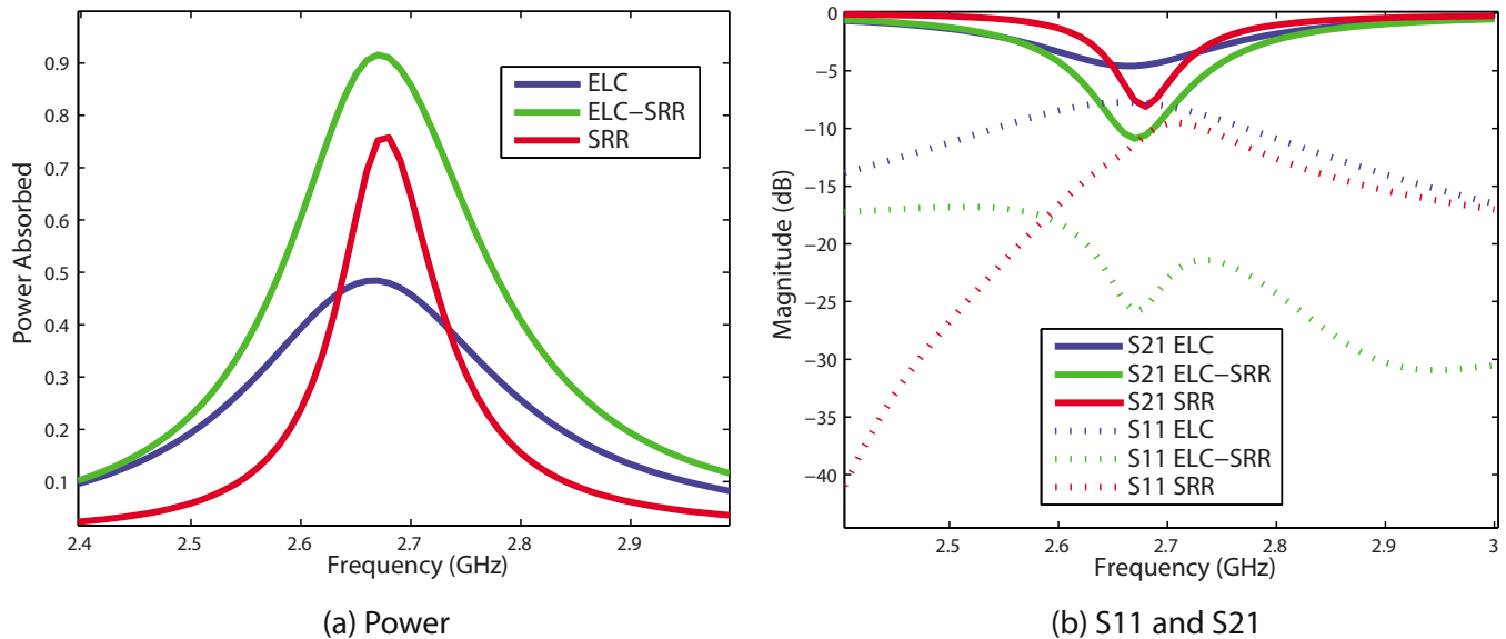
FIG. 3. (Color online) Simulated separate and combined ELC-SRR performance. (a) ELC-SRR absorption is higher and broader than individual ELC and SRR particles. (b) ELC-SRR achieves high absorption through decreased transmission (S21) and low reflection (S11).
