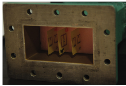
(a) ELC-SRR in WR340 Waveguide
