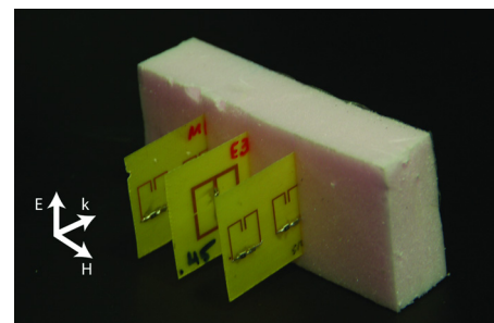
FIG. 2. (Color online) ELC-SRR.
