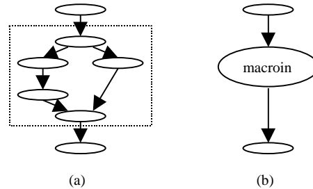
Figure 3: Control Localization (a) control flow graph before control localization. Each oval is an instruction, and the dashed box marks the code sequence to be control localized. (b) control flow graph after control localization
