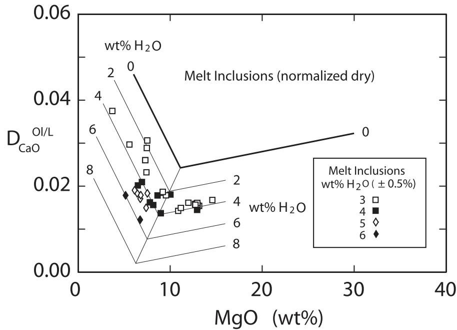
Fig. 7. The distribution of CaO between olivine and coexisting H 2 O–melt inclusions as a function of the melt MgO content. Sources of melt inclusion data are given in the text. The 0 wt % H 2 O isopleth is from Fig. 6a, and the 2–8 wt % H 2 O isopleths are a parameterization of the effects of water on decreasing D_{\text{CaO}}^{\text{Ol/L}} as given in the text. Melt inclusion data are divided between low- and high-MgO populations, separated by the diagonal line as defined by equation (7) in the text.
