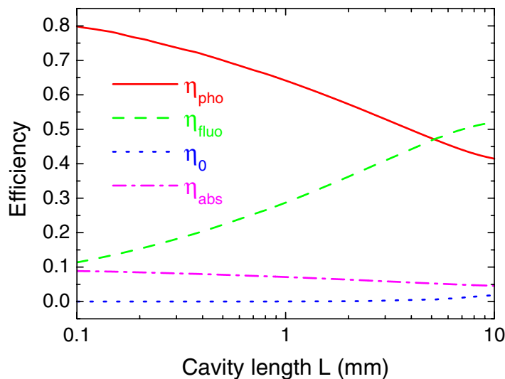
Figure 9. Single-photon efficiency ( \eta_{\text{pho}} ) and probability of fluorescence emission ( \eta_{\text{fluo}} ), ground-state occupation ( \eta_0 ) and photon absorption ( \eta_{\text{abs}} ) as a function of cavity length. The parameters g and \kappa are obtained from figure 8. The pulse length was w = 2500\Gamma_g^{-1} . At each point, \Omega_0 was chosen to optimize the efficiency.
