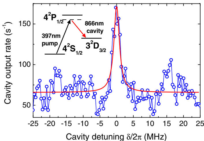
Figure 17. Measurement of the cavity emission as a function of the cavity detuning. The ion is pumped by pulses at 397 nm. Strong cavity output is observed at Raman resonance.
