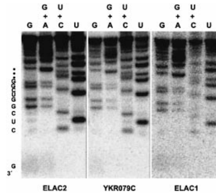
Figure 4. Determination of the exact cleavage site by recombinant 3' tRNases, ELAC2, YKR079C and ELAC1. The unlabeled 5' cleavage products generated in the in vitro 3' tRNase assays were 3'-end-labeled with [5'- 32 P]pCp and T4 RNA ligase, gel-purified and subjected to chemical RNA sequencing (24). The sequencing reactions were analyzed on a 20% polyacrylamide-8 M urea gel. The 3'-terminal nucleotide G corresponds to the discriminator.
