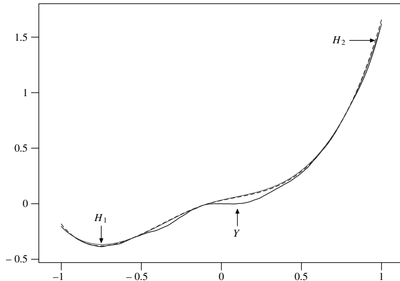
FIG. 1. Y and H_1 , dashed: H_2 . Boundary conditions: f_1(\pm 1) = 12 , f_2(\pm 4) = 192 .
