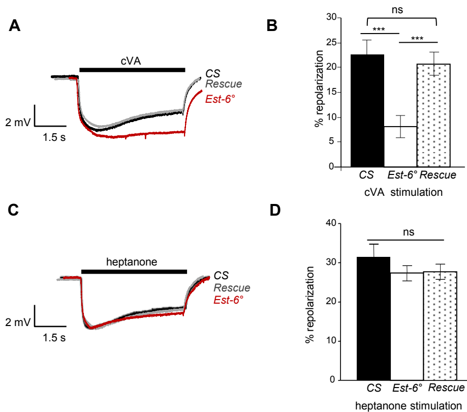
Figure 2 Antennal responses of males to cis -vaccenyl acetate (cVA) and heptanone. (A) Average electroantennography (EAG) plots from wild-type (CS, in black), null mutant ( Est-6° , in red) and rescue ( Rescue , in grey) strains during a 5-s stimulation with cVA. The horizontal bar indicates the duration of stimulus delivery. (B) Percentage of repolarization from the same genotypes calculated at the end of a 5-s stimulation with cVA. Mean \pm SEM; N \geq 10 for each genotype and test. (C) Average EAG plots from CS, Est-6° and Rescue male flies during a 5-s stimulation with heptanone. (D) Percentage of repolarization from the same genotypes calculated at the end of a 5-s stimulation with heptanone. Mean \pm SEM; N = 13 for each test. Student's t test, * P < 0.05 ; ** P < 0.01 ; *** P < 0.001 .
