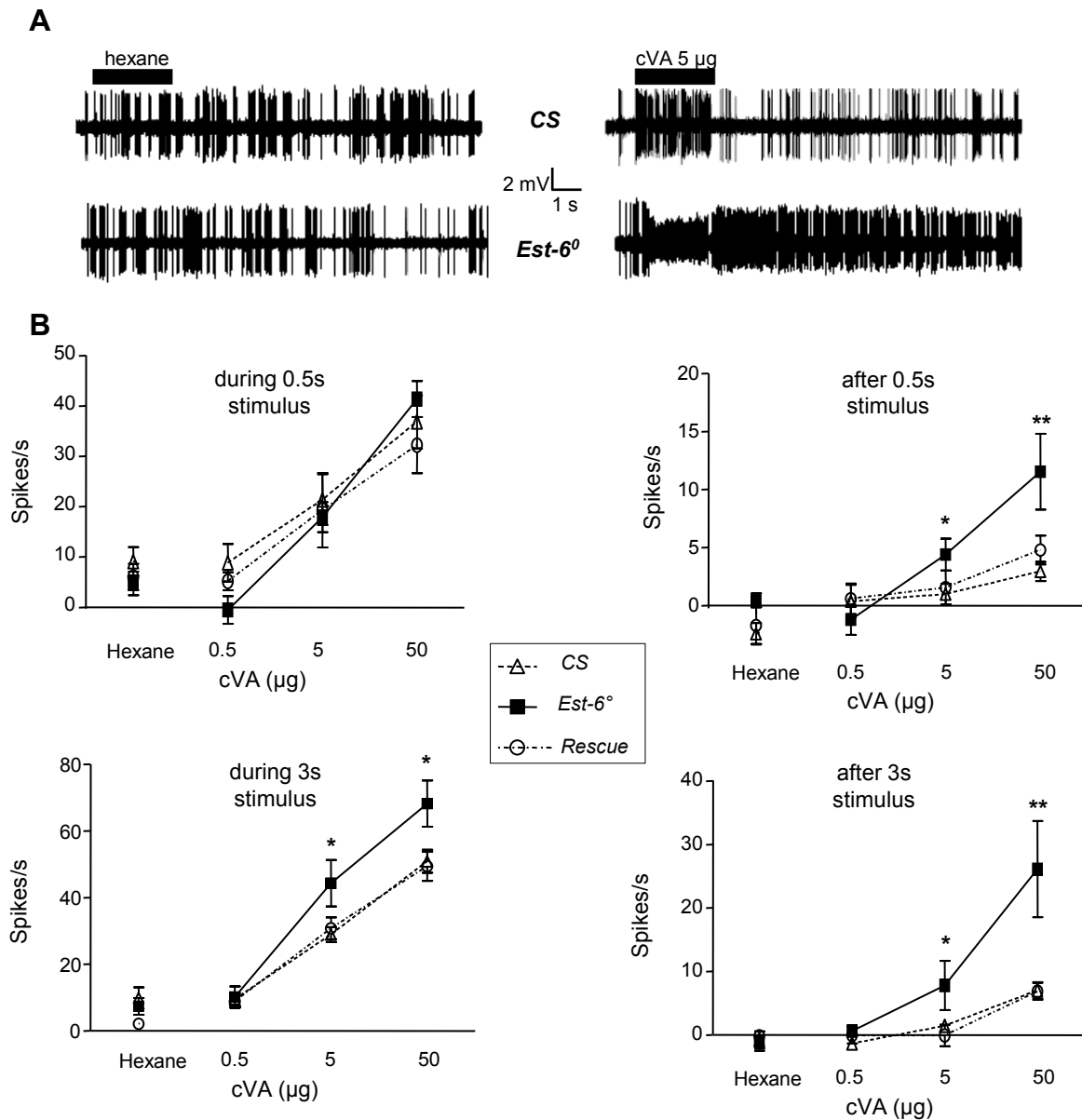
Figure 3 T1 sensillum responses to cis -vaccenyl acetate (cVA) measured by single-sensillum recordings. (A) Action potentials recorded from CS and Est-6° T1 sensilla stimulated for 3 s with solvent (left) or cVA (right). Horizontal bars indicate the duration of stimulus delivery. (B) Dose-response curves for T1 sensilla from CS, Est-6° and Rescue male flies: spike frequencies during the stimulation (0.5 s and 3 s), as well as for 9 s following the stimulus were calculated relatively to the prestimulus frequency. Mean \pm SEM; N \geq 8 for each data point. Student's t test, * P < 0.05 ; ** P < 0.01 .
