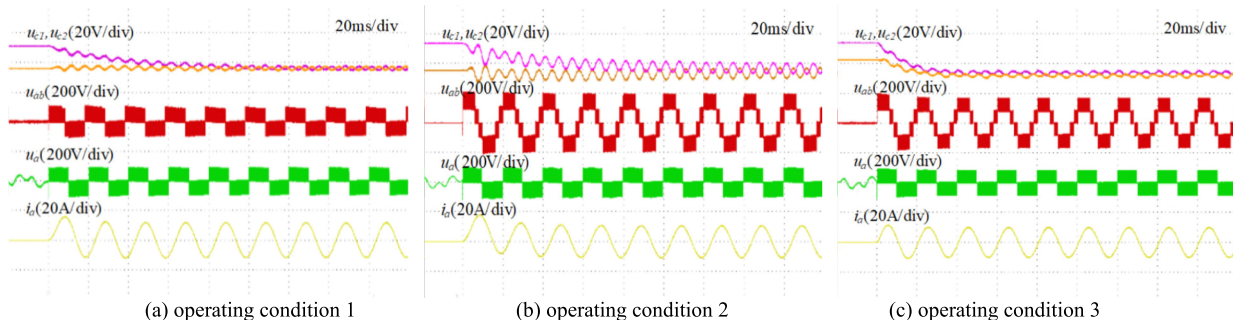
FIGURE 13. The NP voltage recovery ability of SVPWM.
