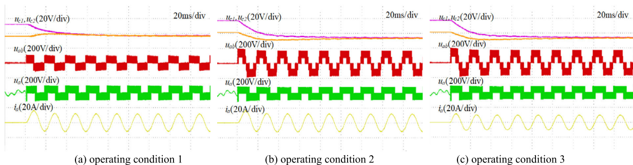
FIGURE 15. The NP voltage recovery ability of VSPWM.
