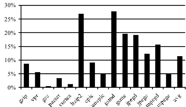
Figure 7: IPC Improvement.
