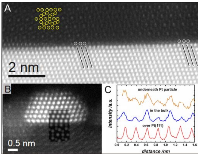
Figure 2. HAADF STEM images of interfaces between: a Pt(111) substrate and an \text{Fe}_3\text{O}_4(111) film (A); an oxide film and a supported Pt particle (B). The Fe atomic columns in the \text{Fe}_3\text{O}_4(111) bulk are marked by circles. Registry variations of the interfacial oxide layer with respect to the Pt(111) surface are highlighted. (C) Intensity profiles measured for the atomic columns in the first oxide layer over a Pt(111) substrate (top), and underneath the Pt particle shown in image B (bottom). The intensity profile along the Kagomé layer in the bulk of the \text{Fe}_3\text{O}_4(111) film is shown for comparison.
