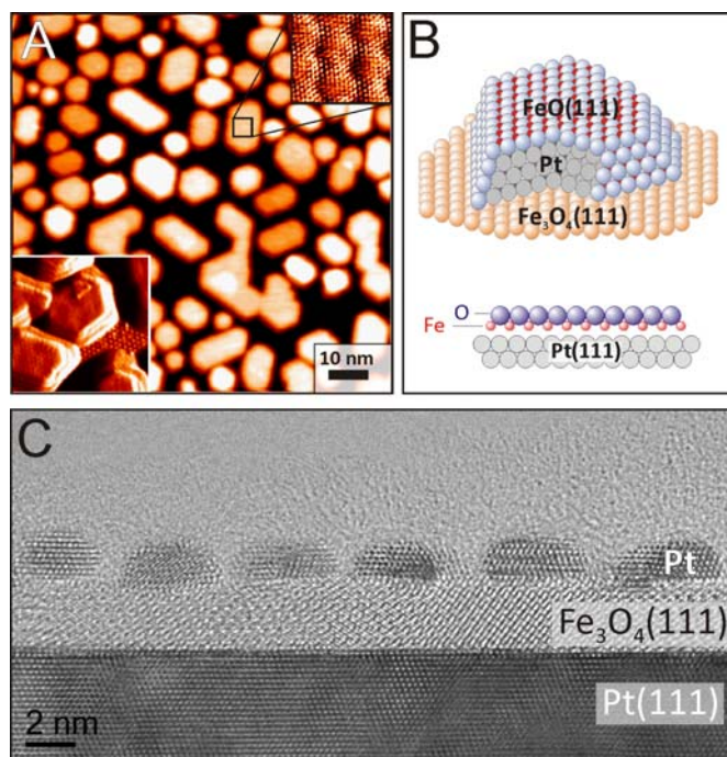
Figure 1. (A) A typical STM image of Pt/Fe 3 O 4 (111) surface after annealing in vacuum at 850 K. (B) Schematic view of an encapsulated Pt particle and a cross-view of an FeO(111) monolayer on Pt(111). (C) High resolution TEM image of Pt/Fe 3 O 4 (111) in the cross-section.
