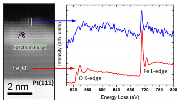
Figure 4. EELS spectra (after baseline subtraction) taken along the line scan as indicated.
