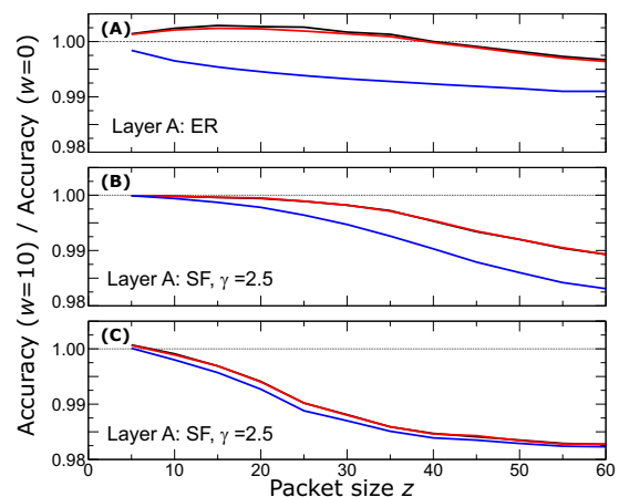
Figure 4. [MODEL 2] (A) Change in accuracy of the ER-layer when it is connected to either an ER layer (black line), a SF layer with \gamma = 2.5 (red), or a SF layer with \gamma = 3.5 (blue), as a function of the packet size z . In all cases, p = 0.3 . (B) Change in accuracy when a SF layer with \gamma = 2.5 is connected to each of the other three layers described above. (C) Same information as above for accuracy in a SF layer with \gamma = 3.5 . Notice that in almost all plots, the black and red lines coincide.
