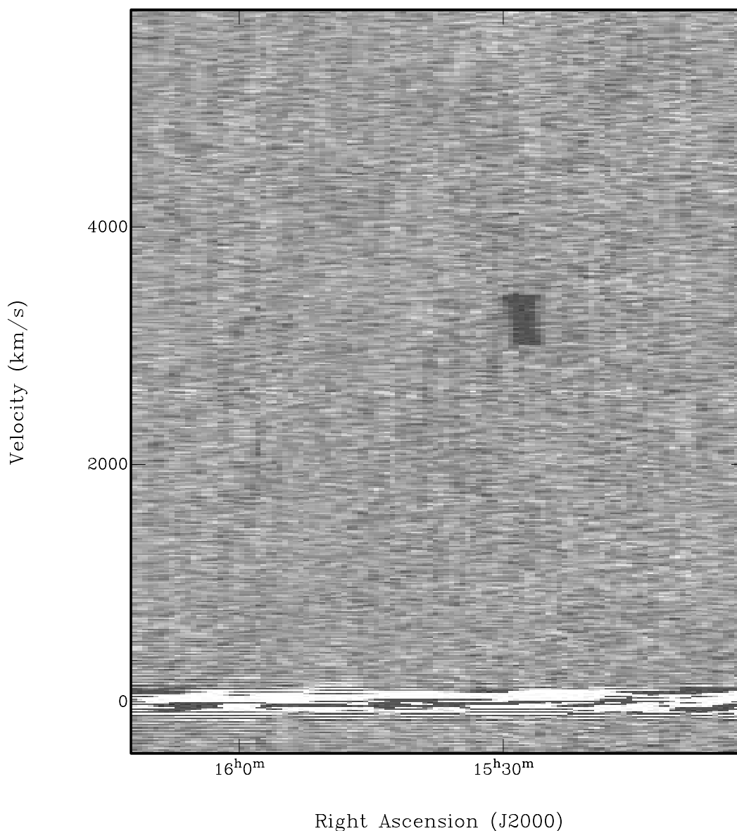
FIG. 1.—Section of a HIPASS data cube at roughly constant declination, -64^{\circ} 11' 58'' 93 (J2000.0). Visible are Galactic H I emission at 0 \text{ km s}^{-1} and the galaxy ESO 099-G005 at \sim 3600 \text{ km s}^{-1} .
