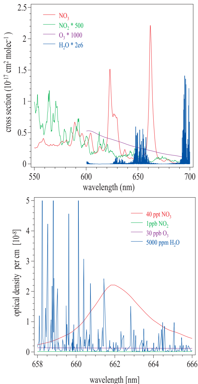
Fig. 3. Upper: NO 3 spectrum compared to other “red” absorbers. The absorption coefficients of NO 2 , O 3 and H 2 O have been scaled upwards as shown. Lower: Result of folding the absorption spectra of NO 3 , NO 2 , O 3 and H 2 O with representative ambient concentrations.
