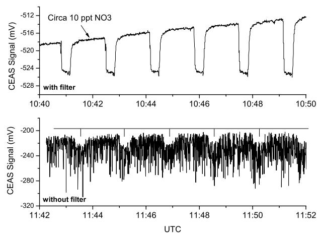
Fig. 4. Upper panel: Raw data obtained in CEAS mode. NO 3 was detected following mixing of NO 2 ( \approx 3 ppbv) and O 3 ( \approx 100 ppbv) in the SAPHIR chamber at 10:30 UT. The difference in signals with and without NO titration correspond to concentrations of NO 3 of between \approx 10 pptv (at 10:40) and 21 pptv of NO 3 (at 10:49) as indicated. The total flow was 3 SLM. Lower Panel: As above, data obtained after removal of filter from inlet. The NO 3 concentration of \approx 50 pptv is barely detectable above a particle induced “noise” of \approx 100 pptv NO 3 equivalents. Note that these concentrations have not been corrected for e.g. inlet/filter loss.
