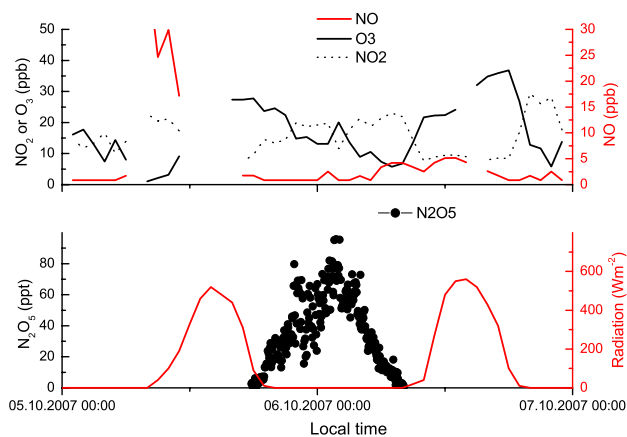
Fig. 10. Upper panel: O 3 , NO and NO 2 mixing ratios reported by the local air monitoring site (≈5 km distance from the MPI building). Lower panel: Data points (left y-axis): N 2 O 5 (+NO 3 ) mixing ratios outside the MPI-building on the night of 5th–6th of October 2007. The solid lines (right y-axis) are global radiation taken from the measurement station of the local (in the state of Hesse) environmental and geological agency.
