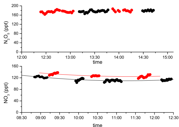
Fig. 8. N 2 O 5 (upper panel) and NO 3 (lower panel) filter transmission tests: Black data points: filter in place, red data points: no filter. The red and black solid lines through the NO 3 data are polynomial fits which guide the eye through the slow changes in the initial NO 3 concentration. For NO 3 , filters with both 1 μm and 2 μm pores were used.
