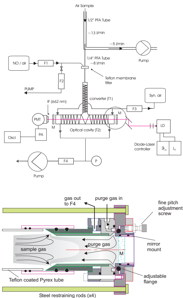
Fig. 1. Schematic/technical diagram of the instrument. F1–4: flow controllers (10, 10, 1000, and 10 000 sccm, respectively), P: pressure gauge, M: 662 nm coated dielectric cavity mirrors, LD: laser diode, IF: interference filter centred at 662 nm, Syn.air: bottled synthetic air for mirror purging, PMT: photomultiplier, Osci: digital oscilloscope for signal acquisition, PA: signal pre-amplifier, NO/air: bottled mixture of 100 ppmv NO in air for \text{NO}_3 titration. The lower section of the figure gives a detailed view of the purge gas in- and outlets and the mirror mounts as enclosed in the dotted circle of the upper section.
