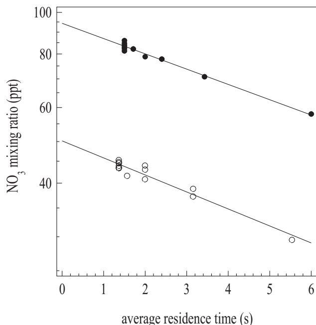
Fig. 6. Determination of NO 3 loss in the inlet lines (PFA-Teflon) and cavity (Teflon FEP 121a coated glass). The two datasets displayed were obtained on separate days (open circles on the 21st, solid circles on the 15th and using two different filters (see text for details). Within experimental uncertainty the decay coefficients were the same.
