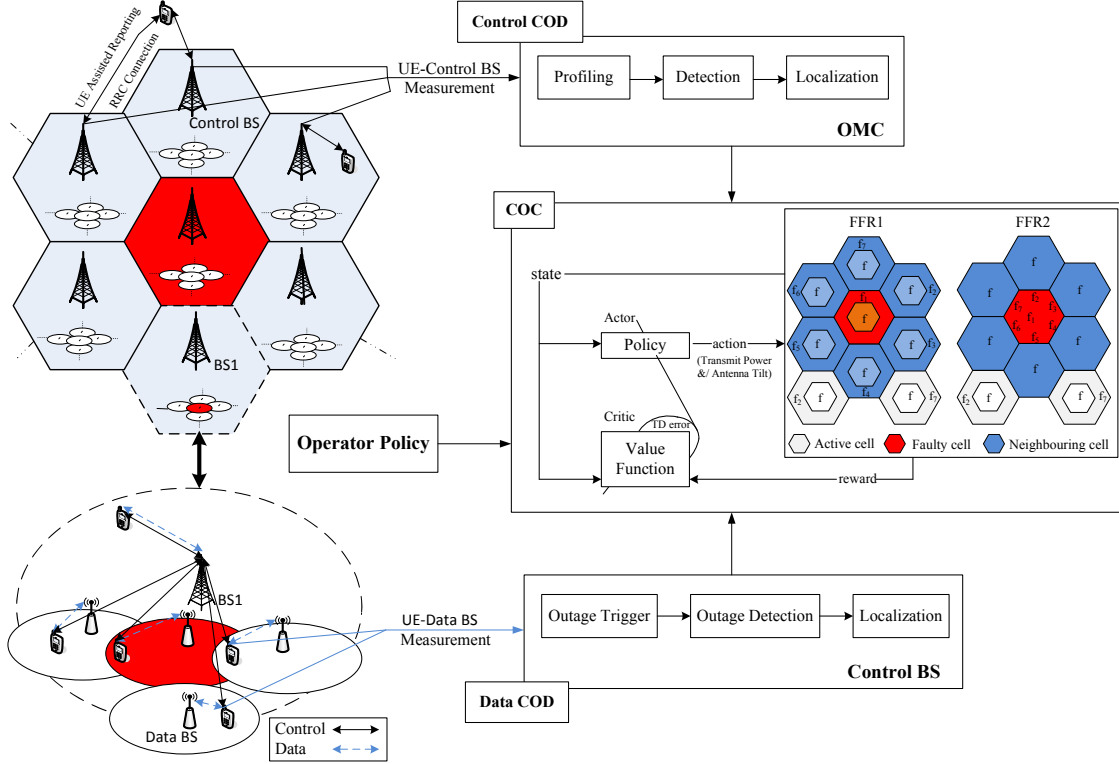
Fig. 1: An overview of COM framework
