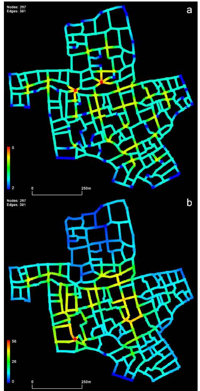
Figure 6. The data and degree distribution.
