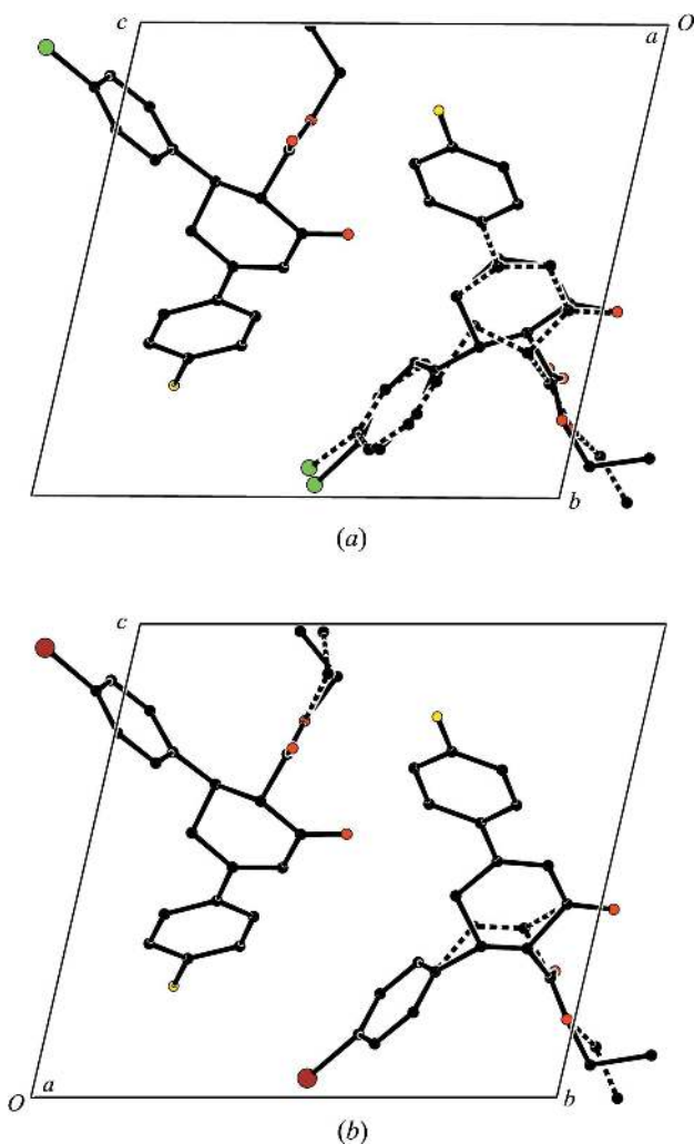
Figure 9 Projections of parts of the crystal structures of compounds (VII) and (VIII), showing the two independent molecules within the unit cells for (a) compound (VII) and (b) compound (VIII). For compound (VII), the original atomic coordinates (Sapnakumari et al. , 2013) were employed, but for compound (VIII) (Kant et al. , 2012), both molecules have been subjected to simple translations within the unit cell. The projections are viewed along [100] and, for the sake of clarity, H atoms have been omitted. Note the different locations of the origin and the different orientations of the unit-cell repeat vectors.
