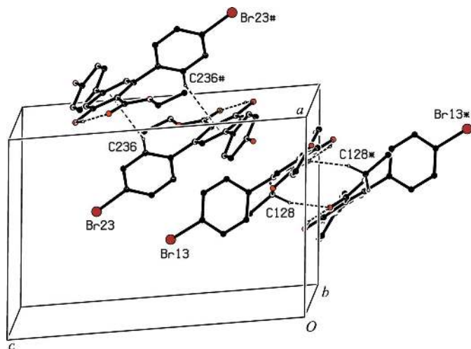
Figure 8 Part of the crystal structure of compound (IV), showing the intramolecular O-H \cdots O hydrogen bonds and the two different hydrogen-bonded dimers formed by the type 1 and type 2 molecules. For the sake of clarity, H atoms bonded to C atoms which are not involved in the motifs shown have been omitted. Atoms marked with an asterisk (*) or a hash (#) are at the symmetry positions (-x+1, -y+2, -z) and (-x+2, -y+1, -z+1) , respectively.
