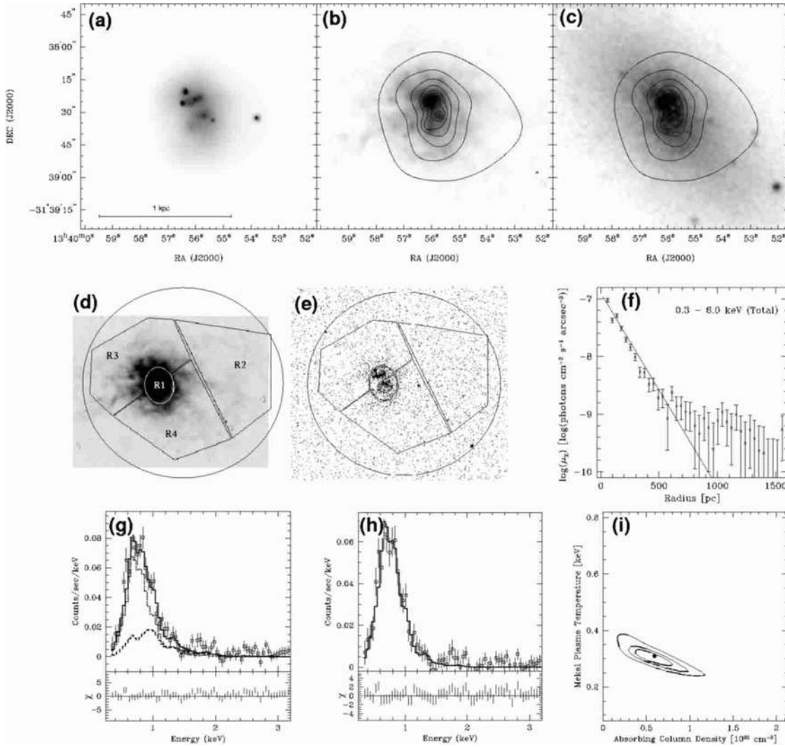
Figure 11. Images and spectra for the X-ray emission of NGC 5253. See the caption of Fig. 3 for details (continuum subtracted H \alpha image taken from Martin 1998, the optical R-band 1.1m ESO Schmidt image from Lauberts & Valentijn 1989).
