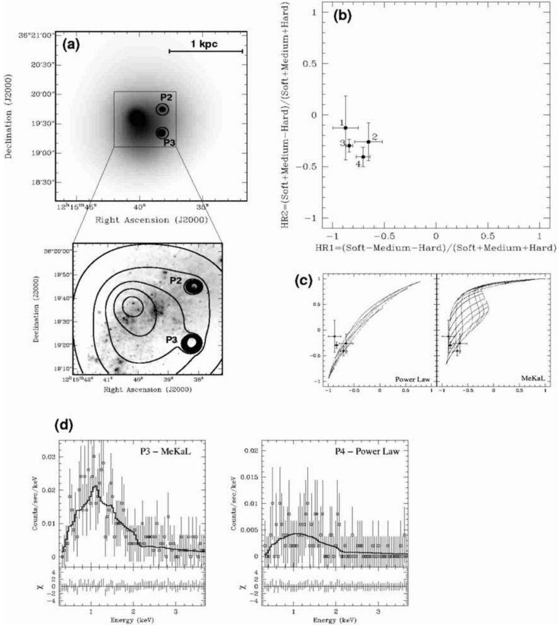
Figure 8. Locations and spectra of the point sources in NGC 4214. See caption of Fig. 4 for details. The count rates, hardness ratios and fitted parameters are listed in Tables 16 and 17.
