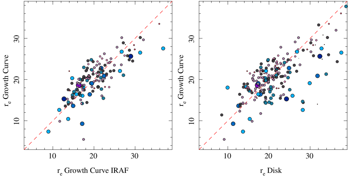
Fig. A.2. Left panel: distribution of the effective radius of the analyzed galaxies, derived from a growth curve analysis (i.e., the total light effective radius), as a function of the same effective radius derived by a similar growth curve analysis using the surface-brightness profiles derived using the ellipse task in IRAF. Right panel: distribution of the effective radius of the analyzed galaxies, derived from a growth curve analysis (i.e., the total light effective radius), as a function of the effective radius of the disk, derived from the exponential fitting to the surface brightness profile. In both panels, larger and bluer symbols correspond to earlier-type galaxies, while smaller and pinky/reddish ones correspond to later type galaxies.
