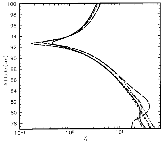
Figure 3. |\eta| for gravity wave with \lambda_x = 100 km, and a period of 20 minutes with dynamics and chemistry (solid line) or dynamics alone (dotted); a period of 1 hour with dynamics and chemistry (dashed-dotted) or dynamics alone (short dashed); and a period of 3 hours with dynamics and chemistry (long dashed) or dynamics alone (dash-triple dotted).
