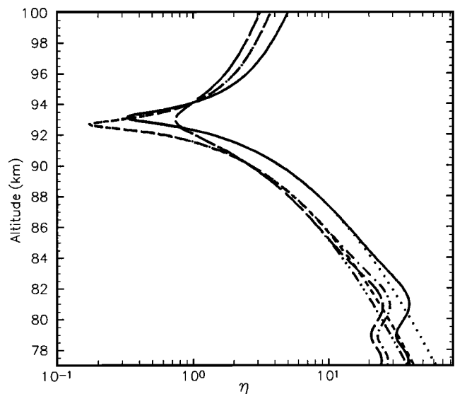
Figure 4. |\eta| for gravity wave with a period of 1 hour, and \lambda_x = 10 km with dynamics and chemistry (solid line) or dynamics alone (dotted); \lambda_x = 100 km with dynamics and chemistry (dashed-dotted) or dynamics alone (short dashed); and \lambda_x = 500 km with dynamics and chemistry (long dashed) or dynamics alone (dash-triple dotted).
