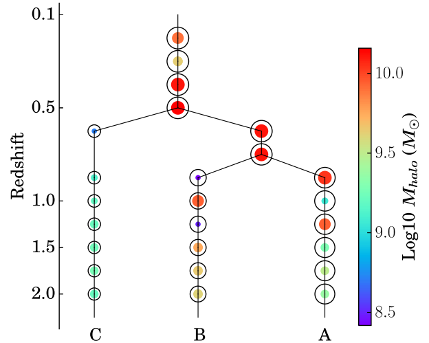
Figure 1. A section of a subhalo merger tree illustrating how subhaloes following branches A and B exchange particles before merging. The colour of the solid symbol reflects the halo mass, while the size of the circle represents the ‘branch mass’, which is the sum of the total mass of all the progenitors sitting on the same branch. A see-saw behaviour is clearly seen in the evolution of the halo mass, which may confuse identification of the most important branch. Instead, we use branch mass to locate the main branch of the tree. In this plot, branch A has the largest branch mass and is therefore chosen as the main branch, even though its progenitors are not always the most massive ones.
