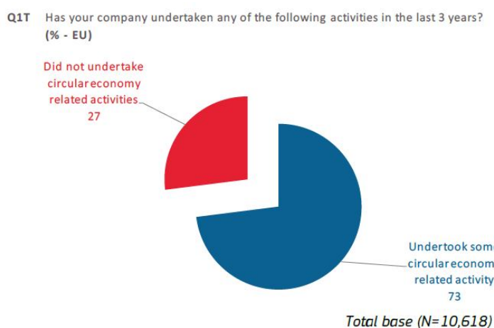
Figure 2 – Results from the EU-level survey [15].
