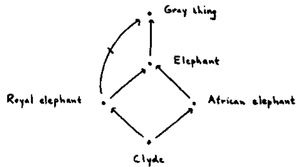
Figure 6: Sandewall's example.
