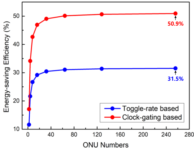
Fig. 11. Energy-saving efficiency of clock-gating and toggle-rate scheme with different ONU numbers.
