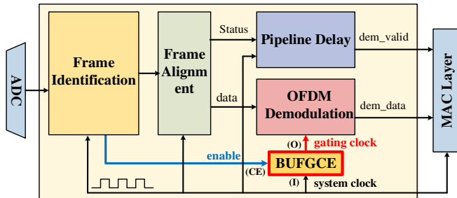
Fig. 2. Real-time OFDM receiver DSP blocks with clock-gating control.
