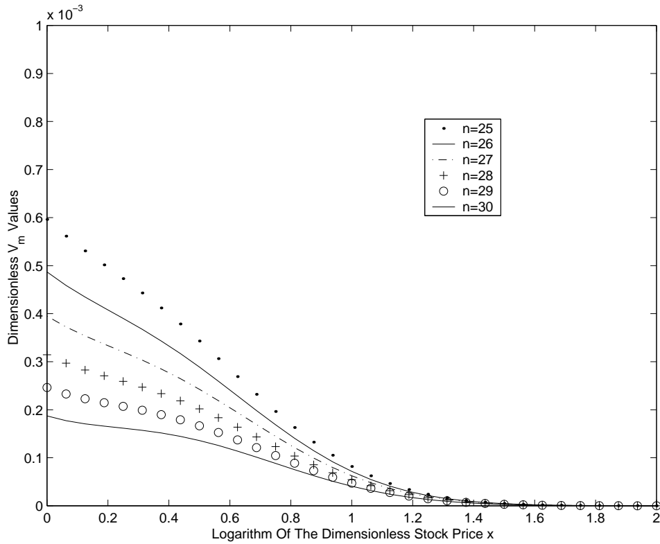
Figure 5: An illustration of convergence for the case with a conversion ratio 0.5
