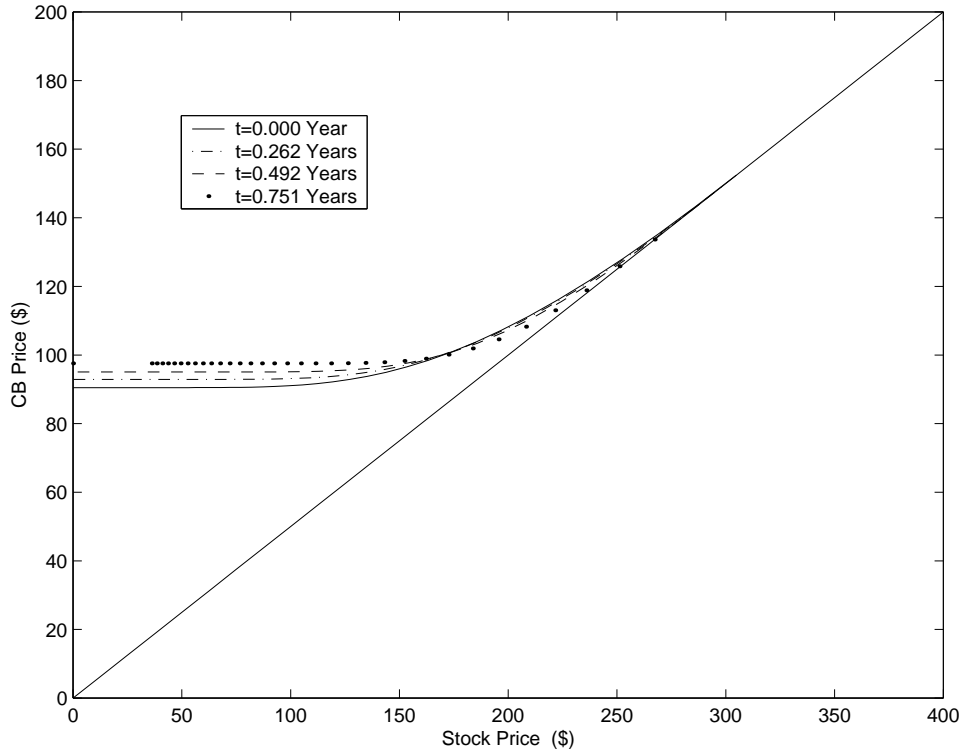
Figure 2: The prices of the convertible bond with a conversion ratio 0.5 at four different time instants
