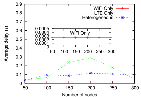
Fig. 8. Packet delays are acceptable for the clustering scheme.
