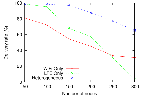
Fig. 6. Packet delivery rate is highest for the clustering scheme.
