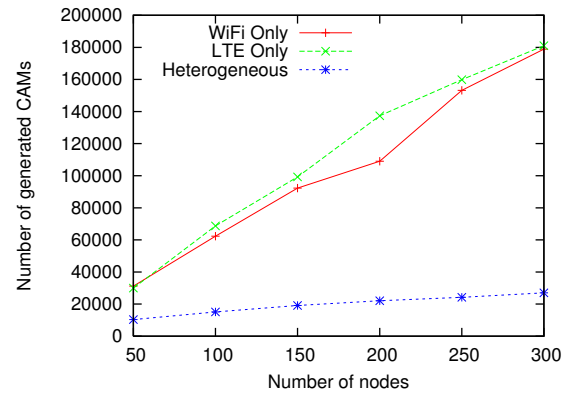
Fig. 7. The number of exchanged CAMs is reduced by clustering.
