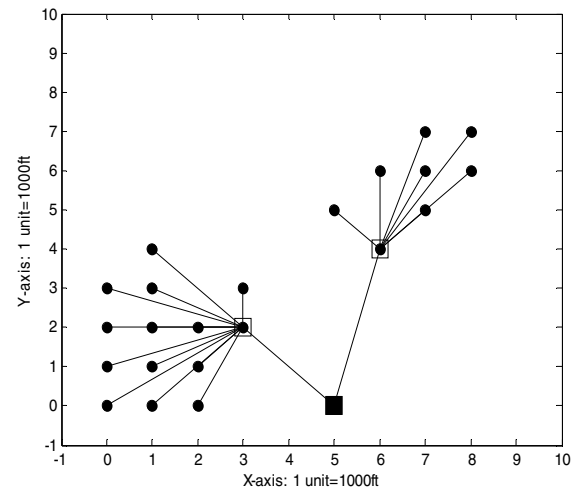
Fig. 6. Mixed layout configuration
