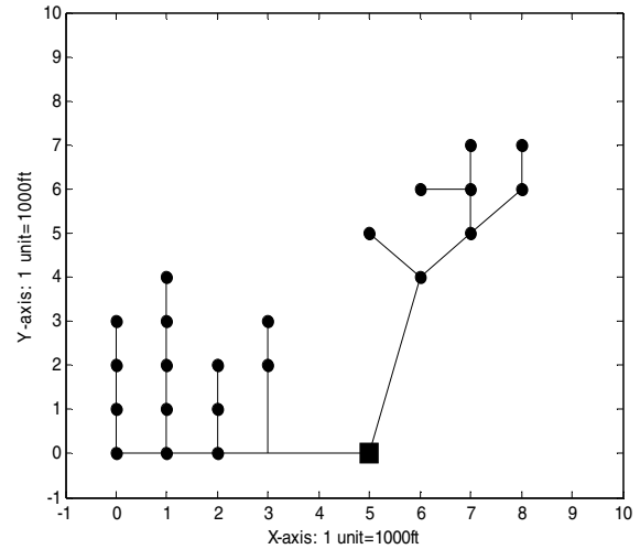
Fig. 5. Radial system cable layout
