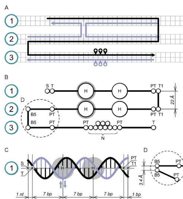
Figure 2. Transition from initial 2D scheme to the COSM model. Blue-encircled numbers specify the index numbers of the corresponding strands. (A) 2D-plot of the DNA origami. Black: scaffold chain; gray-blue: staple chains. Each cell corresponds to one base pair. Sites of insertions are denoted with a tear-shaped sign with a plus symbol; (B) the design from the panel A schematically shown in its COSM representation. The scaffold chain is shown by a black line. Crossover-forming particles are outlined by gray; (C) correspondence between the COSM model for the strand 1 and a B-DNA geometry. COSM particles are in gray, staple crossover site is shown with arrows; (D) an actual geometry of the encircled area from the panel B.
