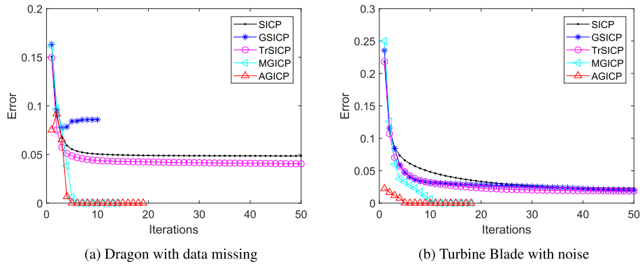
FIGURE 20. RMTSD error for every iteration of SICIP, GSICIP, TrSICIP, MGICP and AGICP, (a) is Dragon data, (b) is Turbine Blade in Fig. 16 and Fig. 17.
