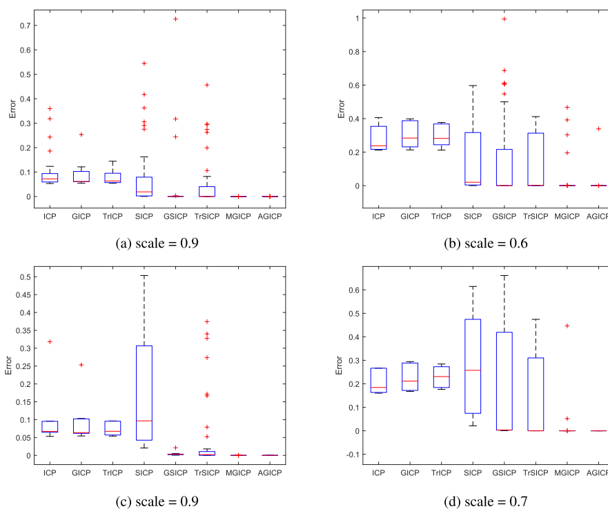
FIGURE 19. Boxplot of RMSD error in various scale cases. (a) and (b) are the results for data with missing data, (c) and (d) are the results for data with noise.
