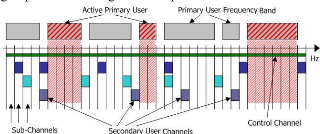
Figure 2. Spectrum pooling idea
