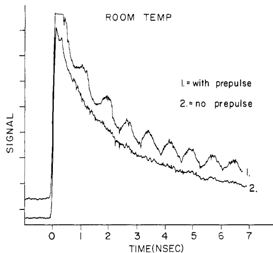
Figure 3. Diffracted signal vs. time for pentacene in p -terphenyl host crystals at room temperature. The upper trace, 1, shows diffraction from both an excited-state grating which decays exponentially and an acoustic grating which gives rise to the oscillations. The lower trace, 2, displays only the excited-state grating. Curve 1 is data taken with the excitation prepulse which populates S_1 . The acoustic grating occurs because of S_1 to S_n absorption of the crossed 532-nm excitation beams. Curve 2 demonstrates that in the absence of the prepulse, all other conditions identical, the normal grating pulse sequence does not produce an oscillatory signal. The amplitude of the oscillations are proportional to the S_1 to S_n absorption cross section at the grating excitation wavelength.
