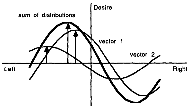
Figure 6-7. Motion commands can be represented by specifying the desirability of various turn angles. The maximum of the combined distributions is the vector sum of the two forces.
