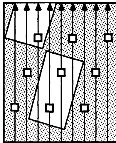
area sampling
