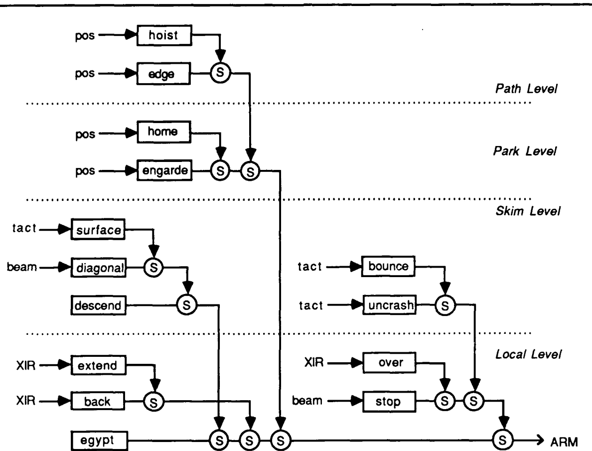
Figure 3-8. The control system for the arm.
