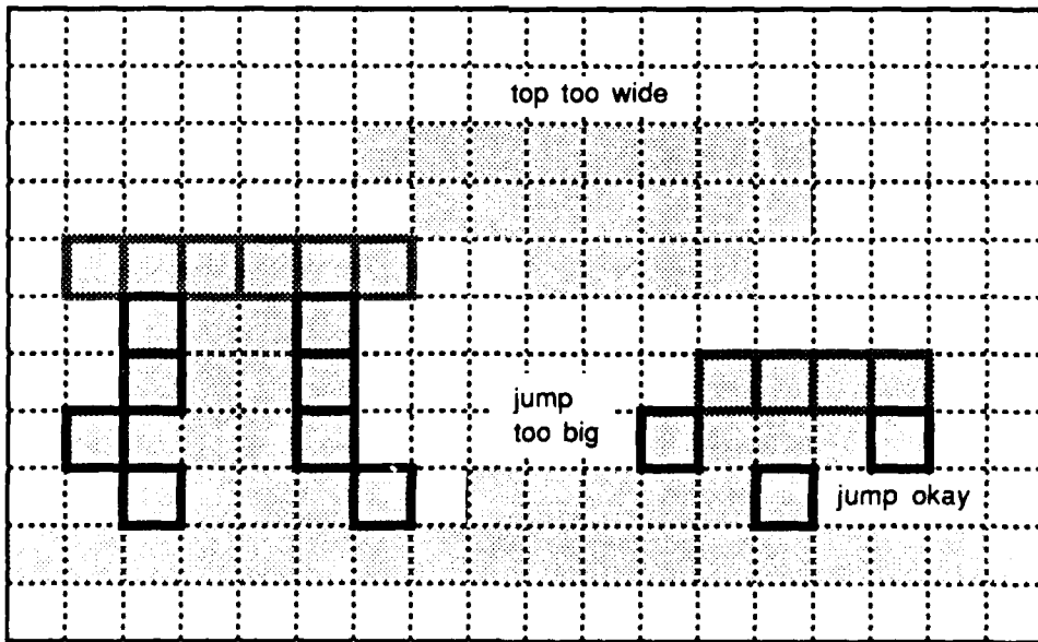
Figure 4-10. The system next looks for medium length horizontal boundaries (dark gray). It marks these as possible can tops and attempts to find approximately vertical adjointed sides (black). If the sides terminate at the same height, a can has been found.
