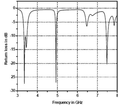
Figure 4. Simulated return loss of the antenna 2.
