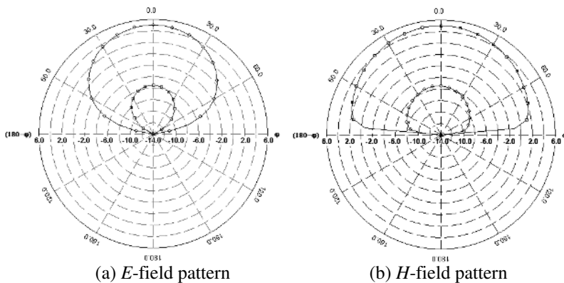
Figure 11. Simulated radiation pattern at 3.45 GHz.
