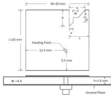
Figure 2. Antenna 2 configuration.
