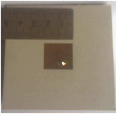
Figure 14. Antenna 1.
