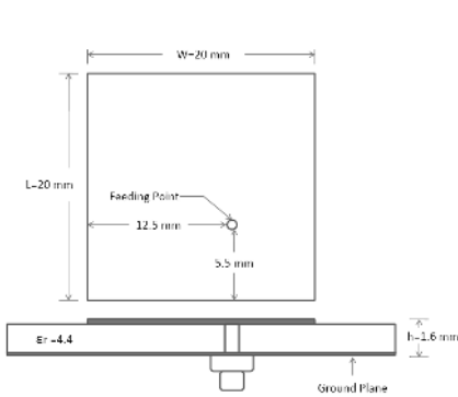
Figure 1. Antenna 1 configuration.
