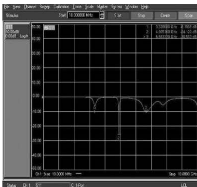
Figure 16. Measured return loss of antenna 1.
