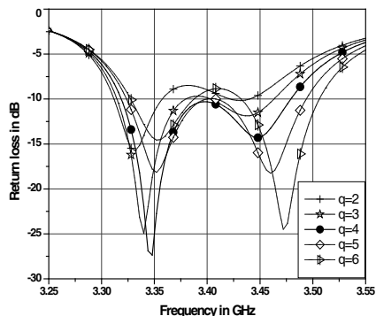
Figure 6. Simulated return loss for different values of q .
