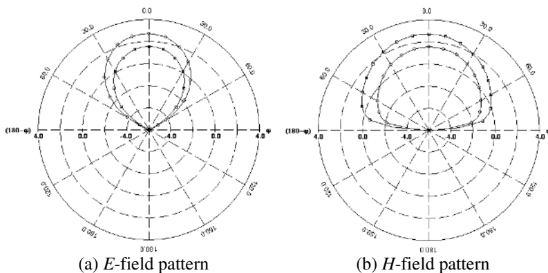
Figure 10. Simulated radiation pattern at 3.4 GHz.
