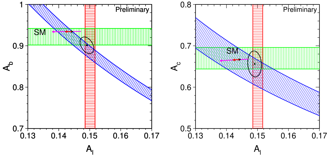
Figure 15.1: The measurements of the combined LEP+SLD \mathcal{A}_\ell (vertical band), SLD \mathcal{A}_b, \mathcal{A}_c (horizontal bands) and LEP A_{FB}^{0,b}, A_{FB}^{0,c} (diagonal bands), compared to the Standard Model expectations (arrows). The arrow pointing to the left shows the variation in the Standard Model prediction for m_H in the range 300_{-186}^{+700} GeV, and the arrow pointing to the right for m_t in the range 174.3 \pm 5.1 GeV. Varying the hadronic vacuum polarisation by \Delta\alpha_{\text{had}}^{(5)}(m_Z^2) = 0.02761 \pm 0.00036 yields an additional uncertainty on the Standard Model prediction, oriented in direction of the Higgs-boson arrow and size corresponding to the top-quark arrow. Also shown is the 68% confidence level contour for the two asymmetry parameters resulting from the joint analyses. Although the A_{FB}^{0,b} measurements prefer a high Higgs mass, the Standard Model fit to the full set of measurements prefers a low Higgs mass, for example because of the influence of \mathcal{A}_\ell .
