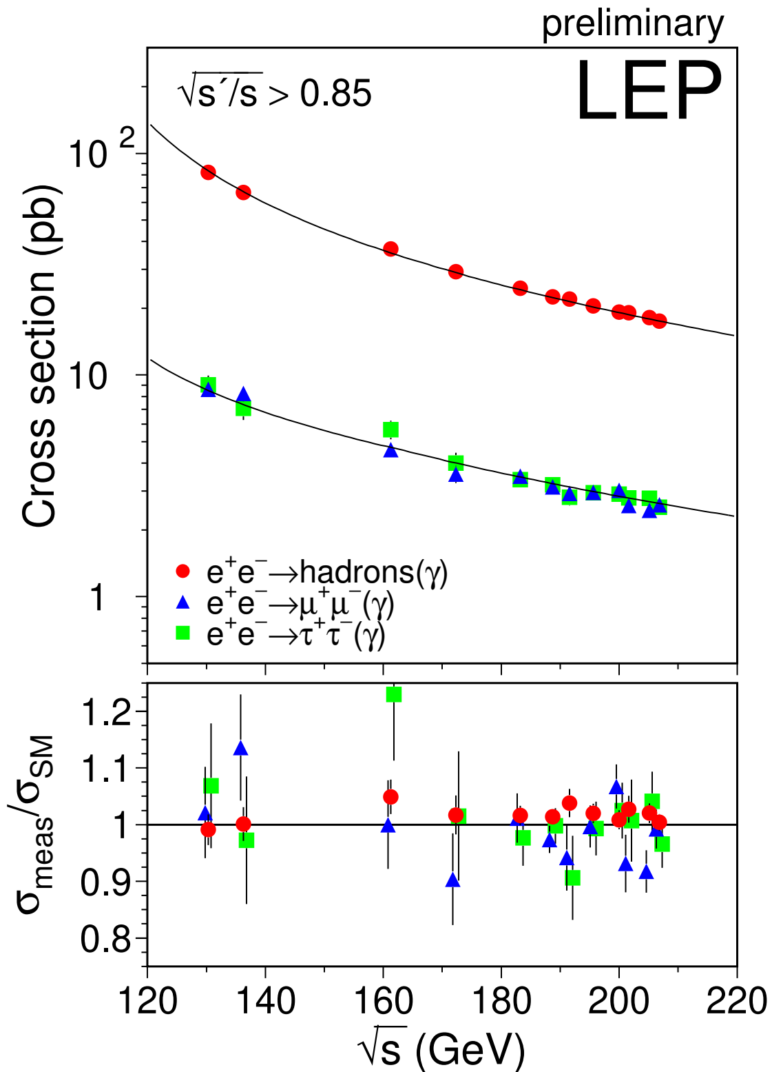
Figure 8.2: Preliminary combined LEP results on the cross-sections for q\bar{q} , \mu^+\mu^- and \tau^+\tau^- final states, as a function of centre-of-mass energy. The expectations of the SM, computed with ZFITTER [84], are shown as curves. The lower plot shows the ratio of the data divided by the SM.
