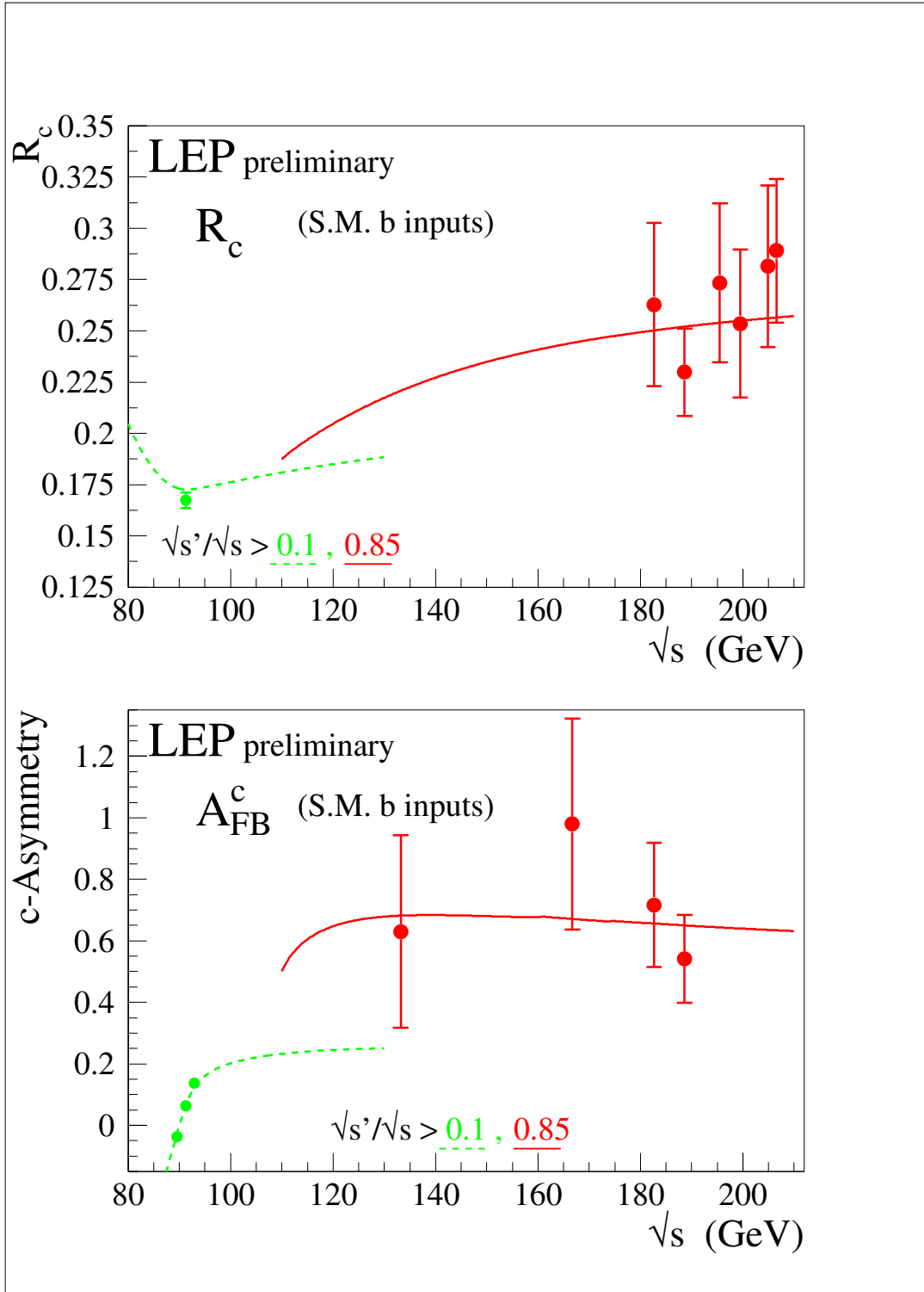
Figure 8.8: Preliminary combined LEP measurements of R_c and A_{\text{FB}}^c . Solid lines represent the Standard Model prediction for the high \sqrt{s} selection used at LEP-II and dotted lines the inclusive prediction used at LEP-I. Both are computed with ZFITTER [90]. The LEP-I measurements have been taken from [91].
