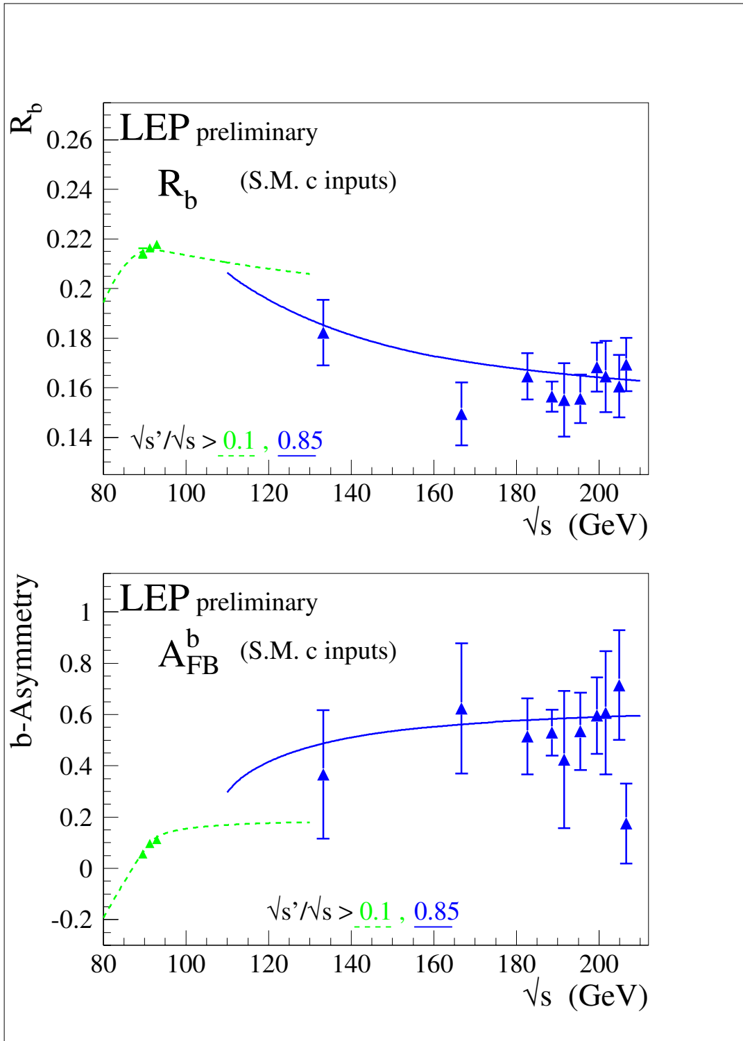
Figure 8.7: Preliminary combined LEP measurements of R_b and A_{\text{FB}}^{b\bar{b}} . Solid lines represent the Standard Model prediction for the high \sqrt{s} selection used at LEP-II and dotted lines the inclusive prediction used at LEP-I. Both are computed with ZFITTER[90]. The LEP-I measurements have been taken from [91].
