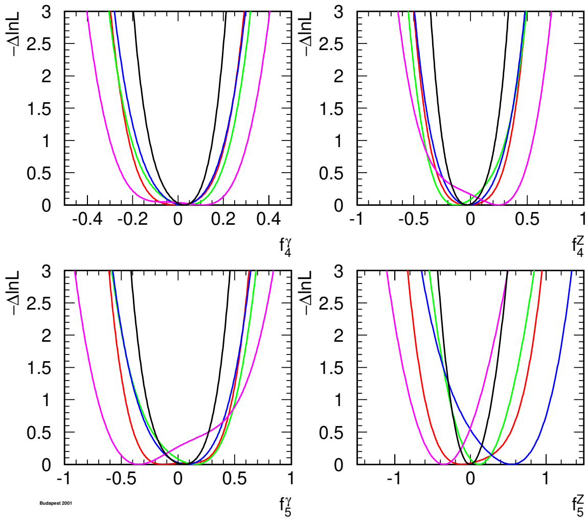
Figure 11.7: The \log \mathcal{L} curves of the four experiments, and the LEP combined curve for the four neutral TGCs f_i^V , V = \gamma, Z , i = 4, 5 . In each case, the minimal value is subtracted.
