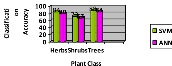
Figure 12: Edge and Edge direction texture features classification accuracy.
