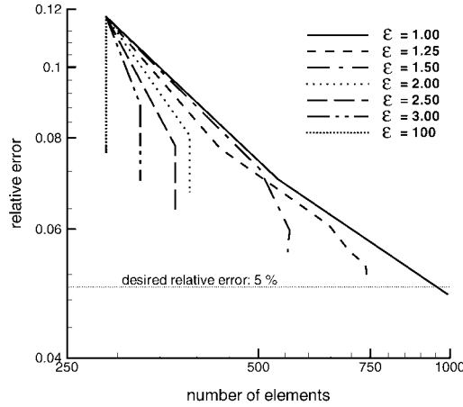
Figure 6. Example of a strip—mesh convergence for different values of \varepsilon .
