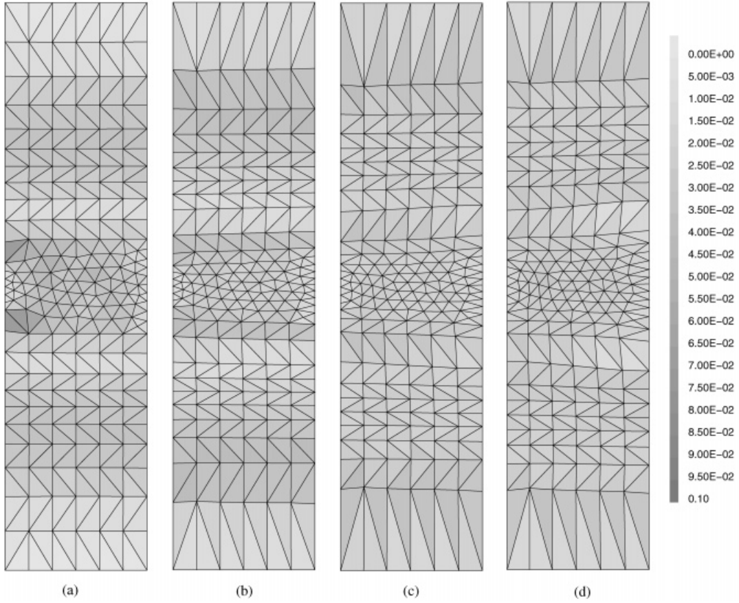
Figure 5. Example of a strip—error distribution after one, two, three and four steps remeshing (a–d, respectively).
