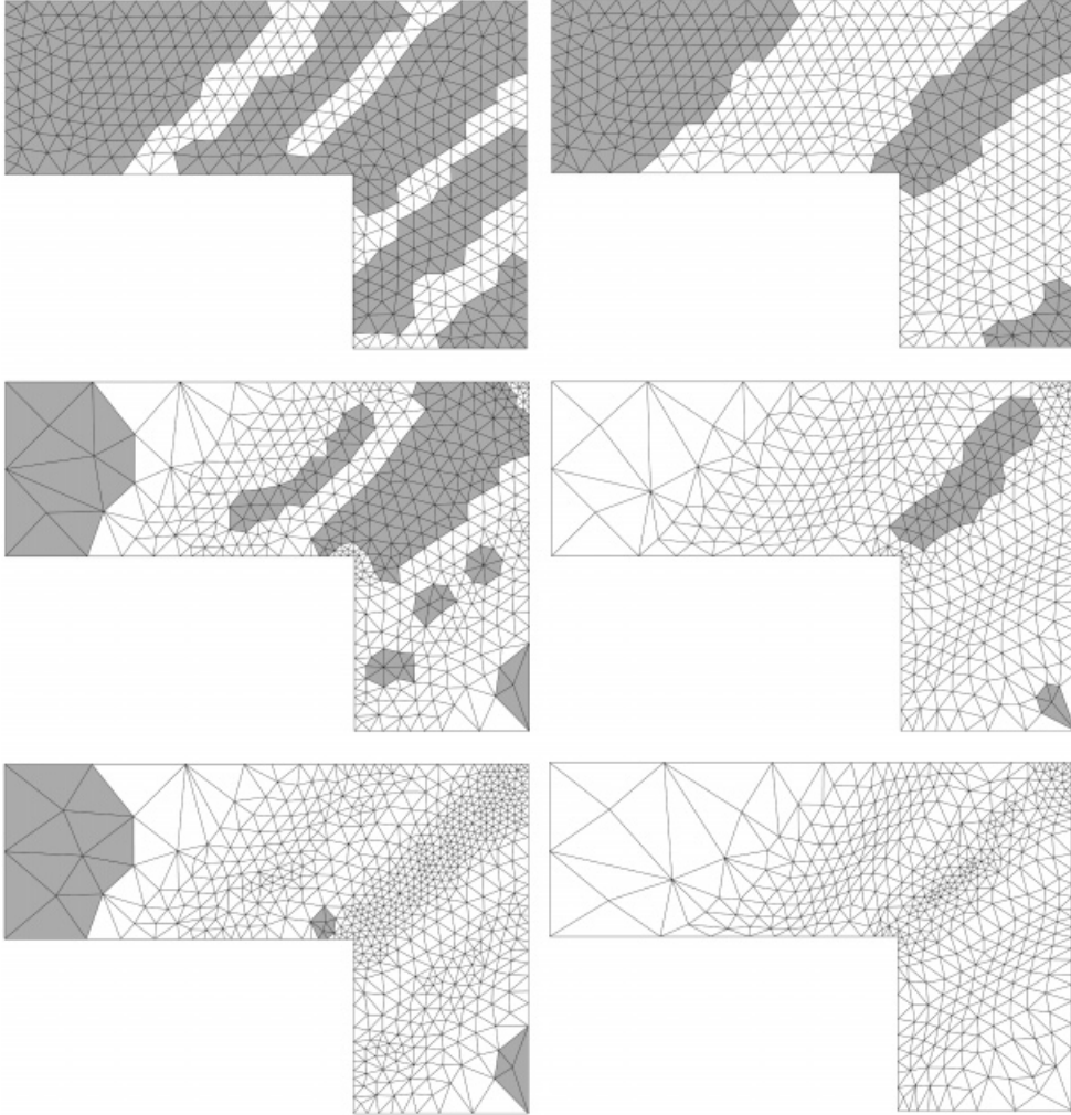
Figure 10. L-shape example—subdivision into h -adaptive subdomain (gray) and r -adaptive subdomain (white) for \varepsilon = 1.5 (left column) and \varepsilon = 2.0 (right column); initial mesh (mesh 0—top row), mesh after one remeshing step (mesh 1—middle row) and mesh after two remeshing steps (mesh 2—bottom row).
