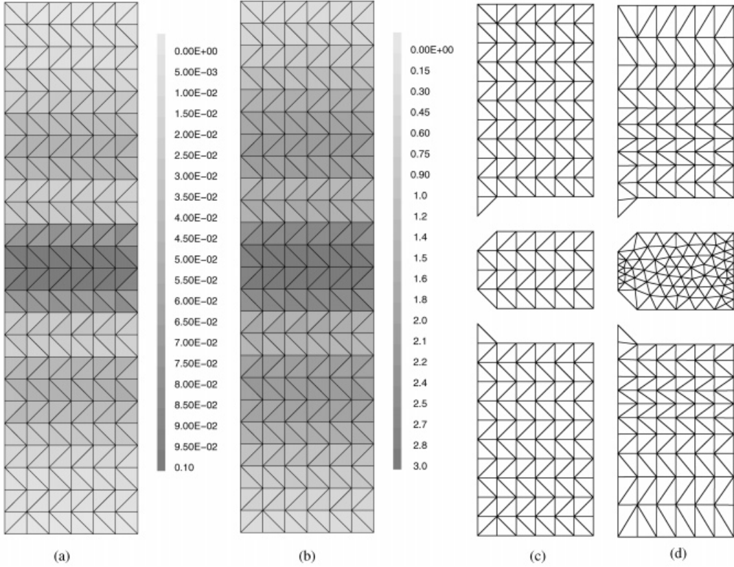
Figure 4. Example of a strip—energy norm of the error (a), refinement ratio (b), splitting the domain (c) and remeshing (d).
