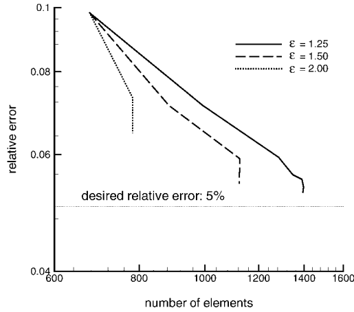
Figure 11. Square with a hole—mesh convergence for fixed values of \varepsilon .
