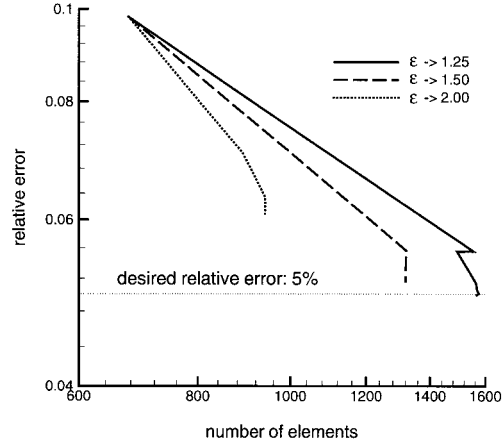
Figure 15. Square with a hole—mesh convergence for an increasing \varepsilon according to Equation (17).
