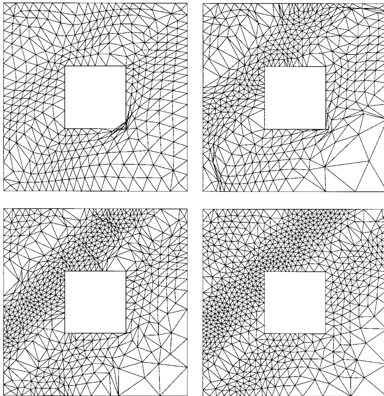
Figure 12. Square with a hole—final meshes for \varepsilon = 100 (top left), \varepsilon = 2 (top right), \varepsilon = 1.5 (bottom left) and \varepsilon = 1.25 (bottom right).
