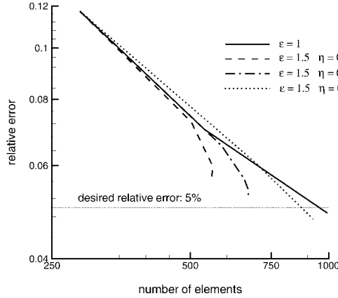
Figure 7. Example of a strip—mesh convergence for different values of \eta .
