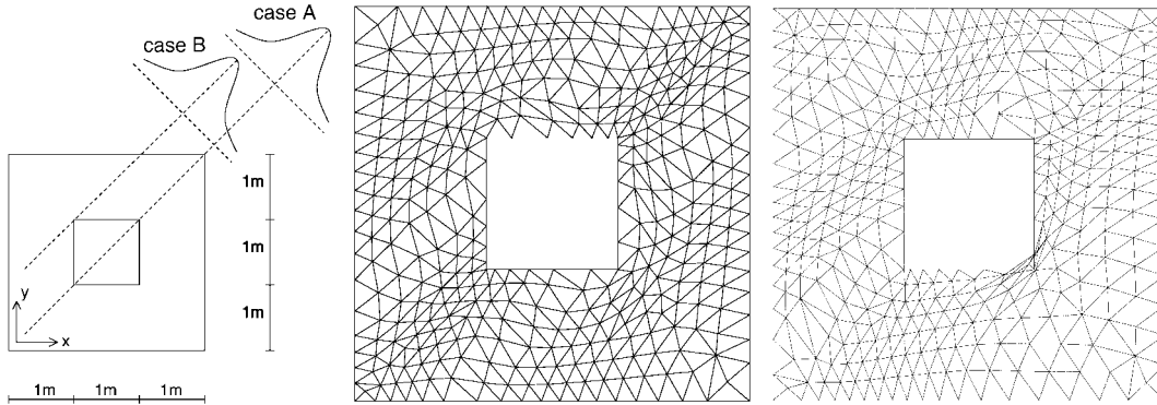
Figure 1. Square with a hole—geometry and temperature fields (left), r -adapted mesh for case A (centre) and r -adapted mesh for case B (right).
