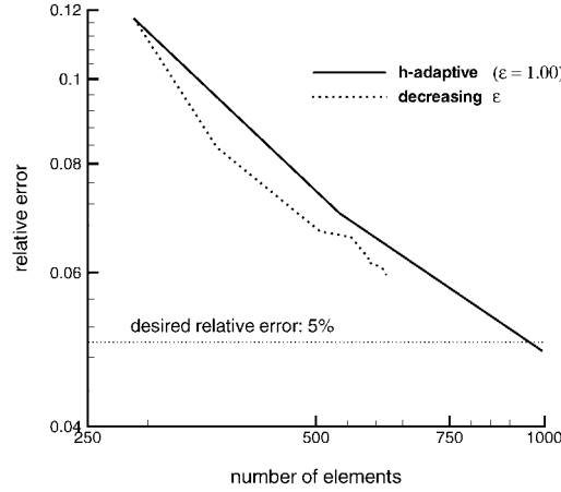
Figure 13. Example of a strip—mesh convergence for a decreasing \varepsilon according to Equation (16).
