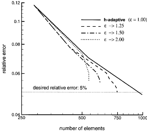
Figure 14. Example of a strip—mesh convergence for an increasing \varepsilon according to Equation (17).
