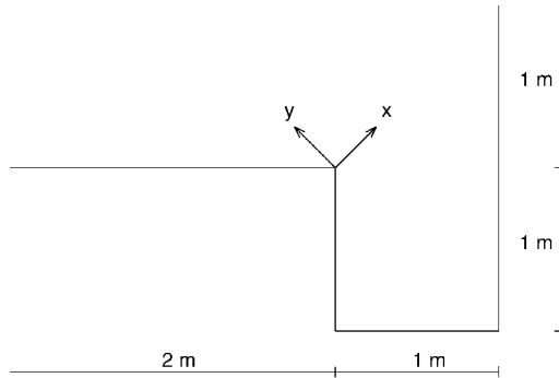
Figure 9. L-shape example—geometry.
