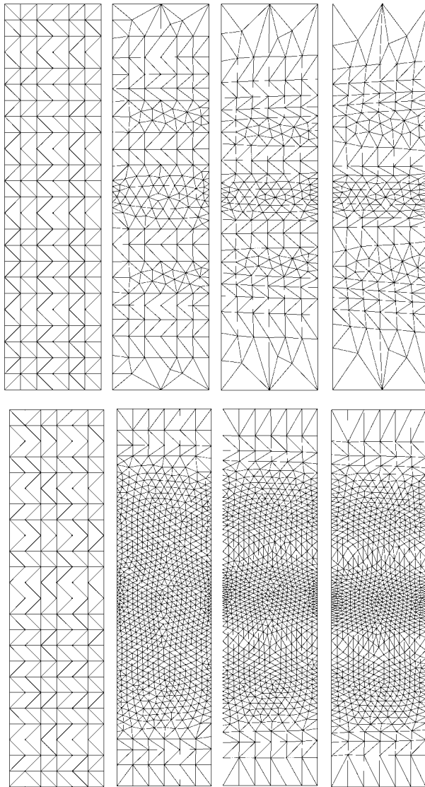
Figure 8. Example of a strip—mesh development for \varepsilon = 2 , prescribed relative error \eta = 0.05 (top row) and \eta = 0.025 (bottom row).
