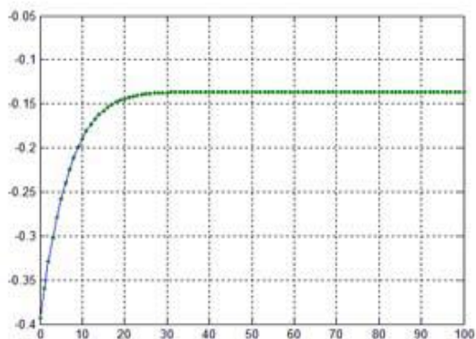
Fig.13 : Orbit of F(z) at s=0.1 and s'=0.5 for (z_0 = -0.3934870291+0i)
