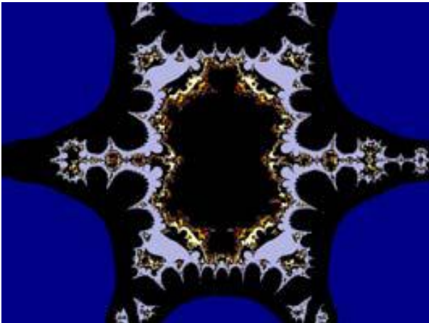
Fig.4 : Relative Superior Mandelbrot Set for s=0.3, s'=0.7
