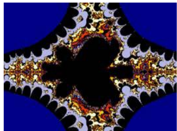
Fig.2 : Relative Superior Mandelbrot Set for s=0.3, s'=0.7
