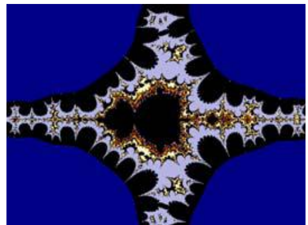
Fig.1 : Relative Superior Mandelbrot Set for s=s'=1
