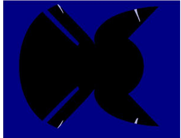
Fig.12 : Relative Superior Julia Set (Tangent Cubic Function) for s=0.9, s'=0.1, c=-0.03352184239-0.03135431148i
