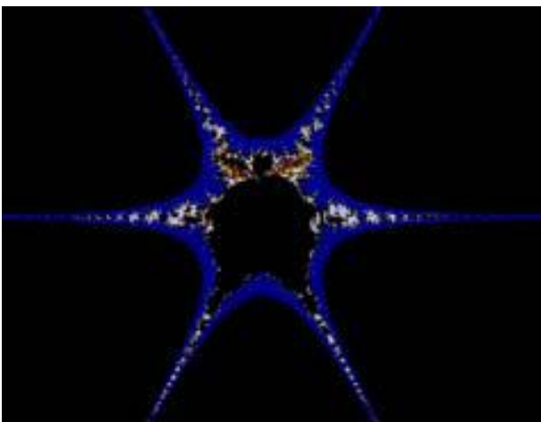
Fig.10 : Relative Superior Julia Set (Sine Cubic Function) for s=0.3, s'=0.7 c= 0.06553079165+1.052110021i
