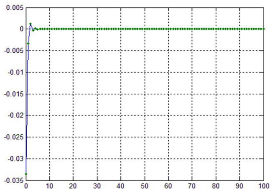
Fig.16 : Orbit of F(z) at s=0.9 and s'=0.1 for (z_0=-0.03352184239-0.03135431148 i)
