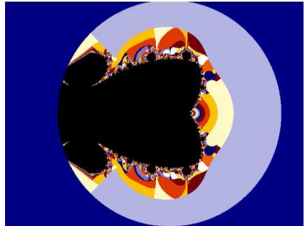
Fig.6 : Relative Superior Mandelbrot Set for s=0.9, s'=0.1
