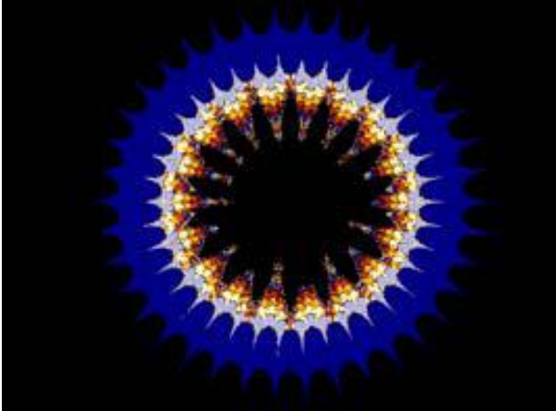
Fig.9 : Relative Superior Mandelbrot Set for s=0.1, s'=0.5 n=19
