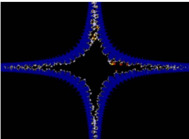
Fig.10 : Relative Superior Julia Set (Sine Cubic Function) for s=0.3, s'=0.7 c= 0.06553079165+1.052110021i
