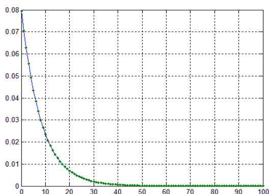
Fig.14 : Orbit of F(z) at s=0.1 and s'=0.5 for (z_0 = 0.07944042258+0.03670696339i)
