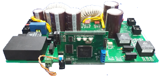
Fig.9 Prototype of the proposed converter.
