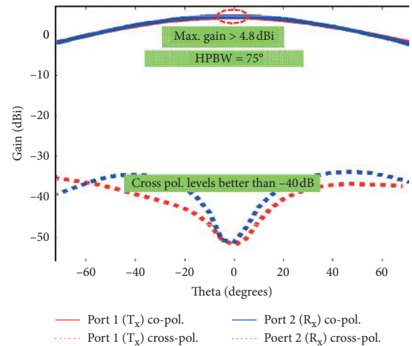
FIGURE 8: The measured T_x and R_x modes copolarization and cross-polarization gain levels for the presented antenna at 2.405 GHz frequency.
