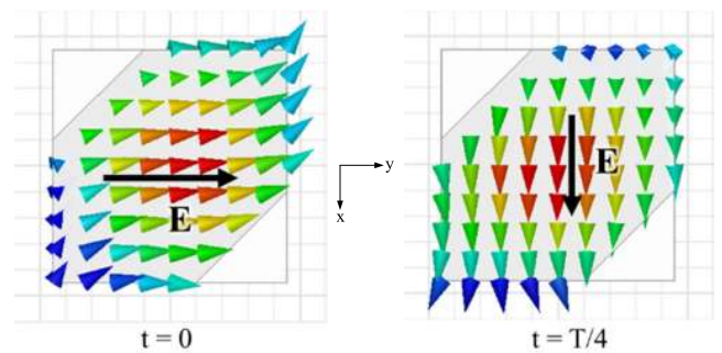
FIGURE 4. E-field distribution at the top of the DR for time period T at 3.45 GHz.
