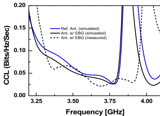
FIGURE 26. Comparison of channel capacity loss (CCL) for antenna with and without EBG.
