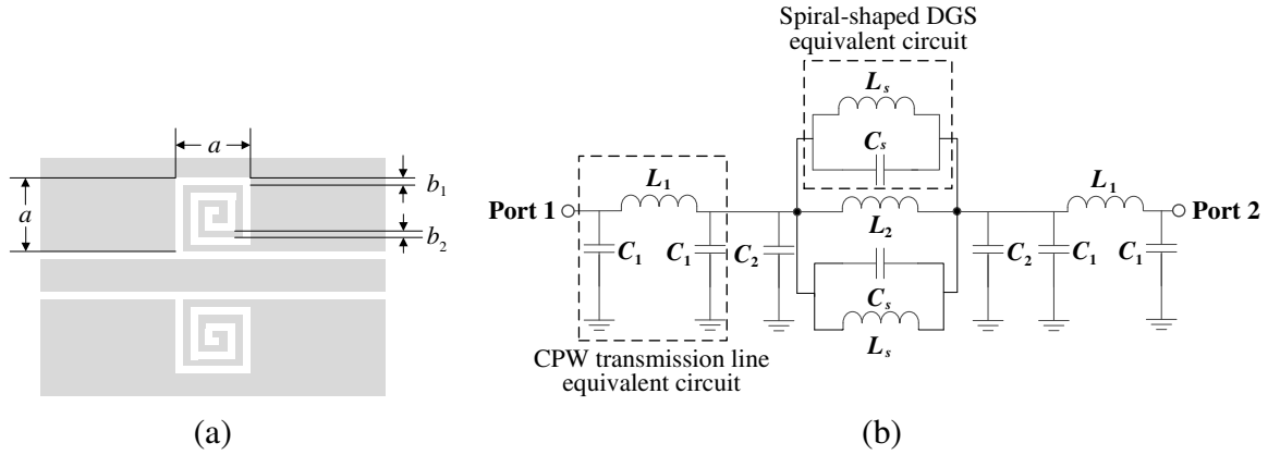
Figure 1. A section of spiral-shaped DGSs. (a) Layout. (b) Equivalent circuit.
