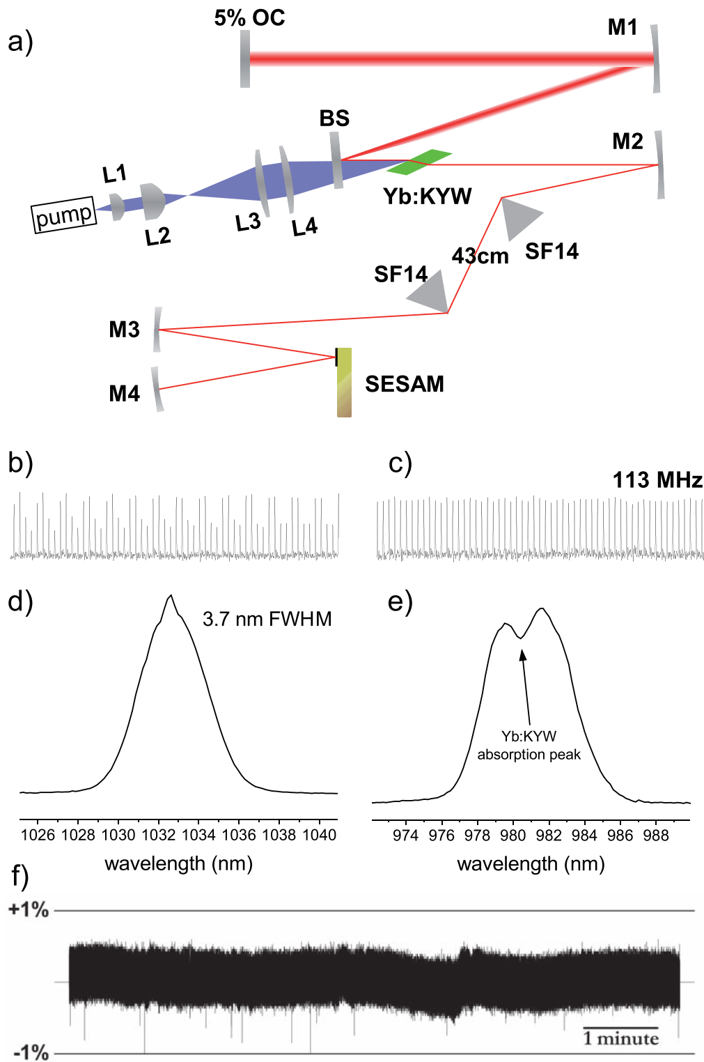
Figure 2. Design and performance of the Yb:KYW laser. a) Diagram of the laser cavity. Pump light is collimated and focused by lenses L1–4 to a 51 \mu\text{m} \times 85 \mu\text{m} waist in air; pump beam is tilted relative to the lasing beam to keep reflections from reentering the pump diode and destabilizing it. Beamsplitter (BS) has high transmissivity at 981 nm and high reflectivity at >1010 nm. Lasing medium is a d=1.2 mm Brewster-cut 10%-at. Yb:KYW crystal. M1, M4 = -200 mm, M2, M3 = -100 mm are cavity mirrors with standard \lambda/4 dielectric coating. SF14 – uncoated isosceles prisms. OC – output coupler. b) Low pump beam quality makes the laser prone to multimode operation, which is easily observed by a photodiode as the circulation of pulse energy between lobes of higher-order modes on subsequent passes. c) Restricting the cavity to single-mode operation results in even pulsing at 113 MHz with 300 mW of average power. d) Output spectrum is 3.7 nm wide and centered near 1033 nm, indicating sech 2 transform-limited pulse width of 310 fs. e) Spectrum of the transmitted pump light. The narrow Yb:KYW absorption peak near 981 nm is readily visible; the pump wavelength must be temperature-tuned to overlap it for maximum output power and stability. f) Output power variability. With the off-axis pumping arrangement the laser is capable of very quiet operation. doi:10.1371/journal.pone.0000699.g002
