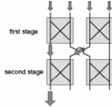
Figure 2. Schematic of hybrid arrangement for combining and directing four input signals to any of four outputs.
