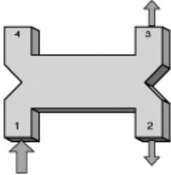
Figure 1. H-planar geometry of the magic H hybrid. Power-flow arrows illustrate splitting function (reverse for combining).
