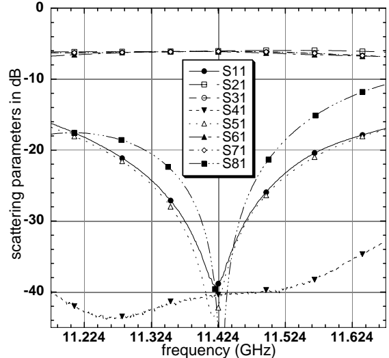
Figure 4. Measured amplitudes, in dB, of the first column scattering matrix elements (and by symmetry all others) for the cross potent superhybrid over a frequency range of 500 MHz centered on 11.424 GHz.
