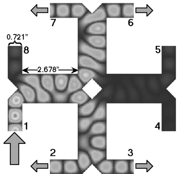
Figure 3. H-planar geometry of an eight-port cross potent superhybrid. Power-flow arrows and an HP HFSS electric field plot illustrate four-way splitting function with power fed into port 1 (reverse for combining).
