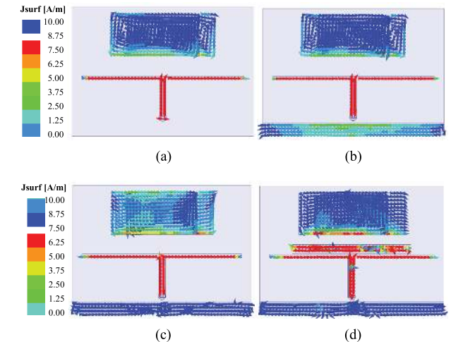
FIGURE 4. Surface current distributions on reference Antennas I, II, and III. (a) Antenna I at 1.65 GHz. (b) Antenna II at 1.65 GHz. (c) Antenna II at 3.03 GHz. (d) Antenna III at 3.03 GHz.
