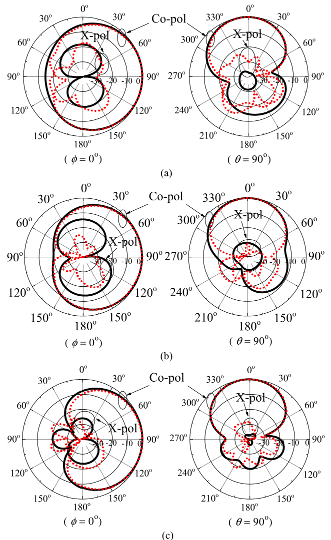
FIGURE 11. Simulated and measured radiation patterns of the prototype. (a) 2.08 GHz. (b) 2.34 GHz. (c) 2.64 GHz. — Simulated ····· Measured.
