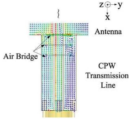
Fig. 7. HFSS-simulated current distribution at the intersection between the antenna terminal and the CPW feedline under the dipole mode of operation.
