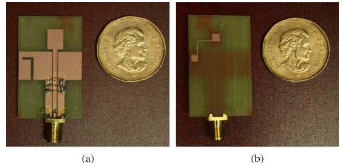
Fig. 10. The fabricated prototype of the tri-band monopole antenna with single-cell MTM loading and a “defected” ground-plane. (a) Front side. (b) Back side.
