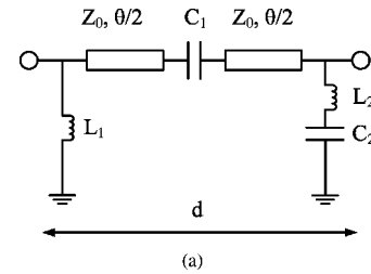
Fig. 3. The equivalent circuit when the proposed tri-band antenna operates at the monopole mode. The dimension d refers to the size of the NRI-TL unit cell and it corresponds to roughly the length of the monopole L_m with reference to Fig. 1(a).
