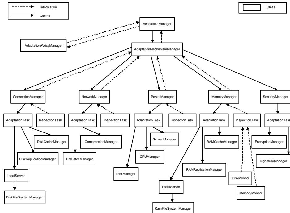
Fig. 2. The proposed reflective middleware architecture
