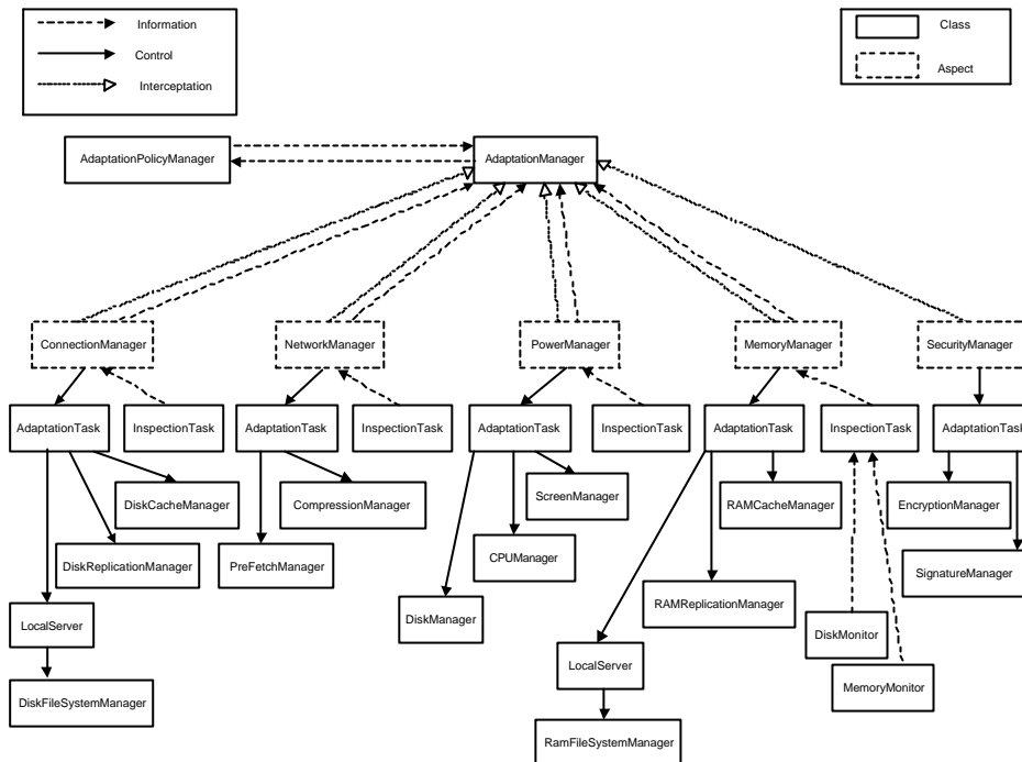
Fig. 5. The proposed aspect oriented middleware architecture
